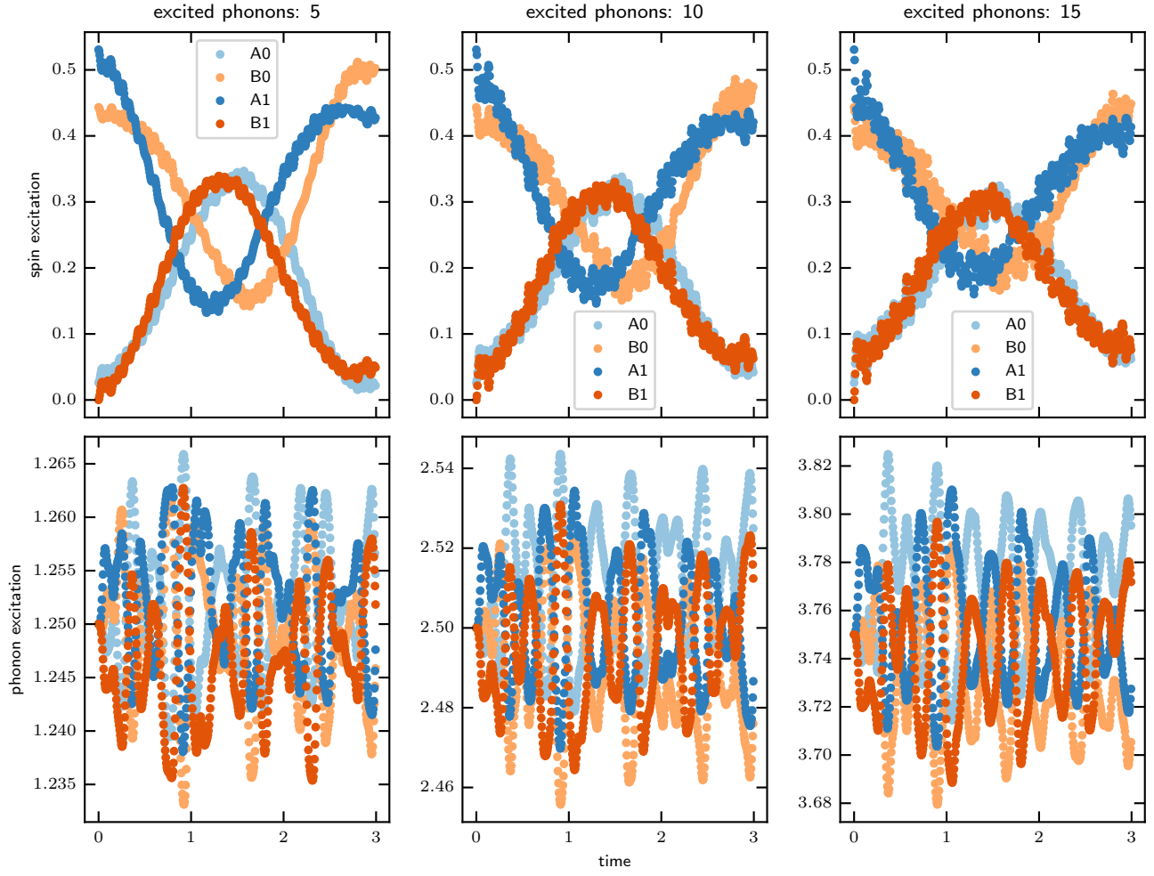
Figure 14: Evolution with full Hamiltonian ratio spin only: coupling 1:10.
