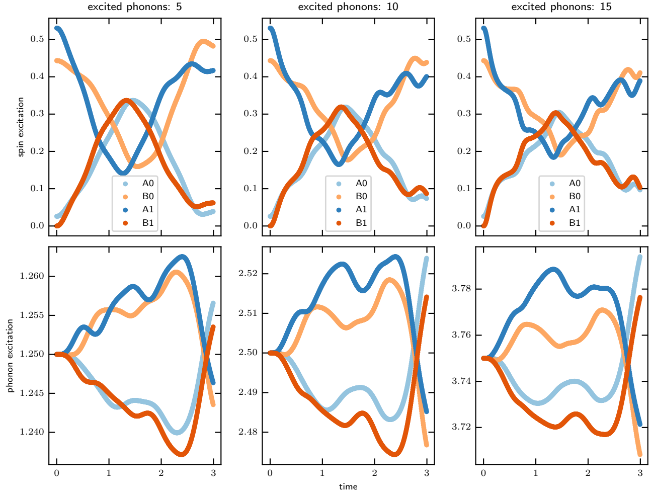
Figure 13: Evolution with full Hamiltonian ratio spin only: coupling 1:1.
