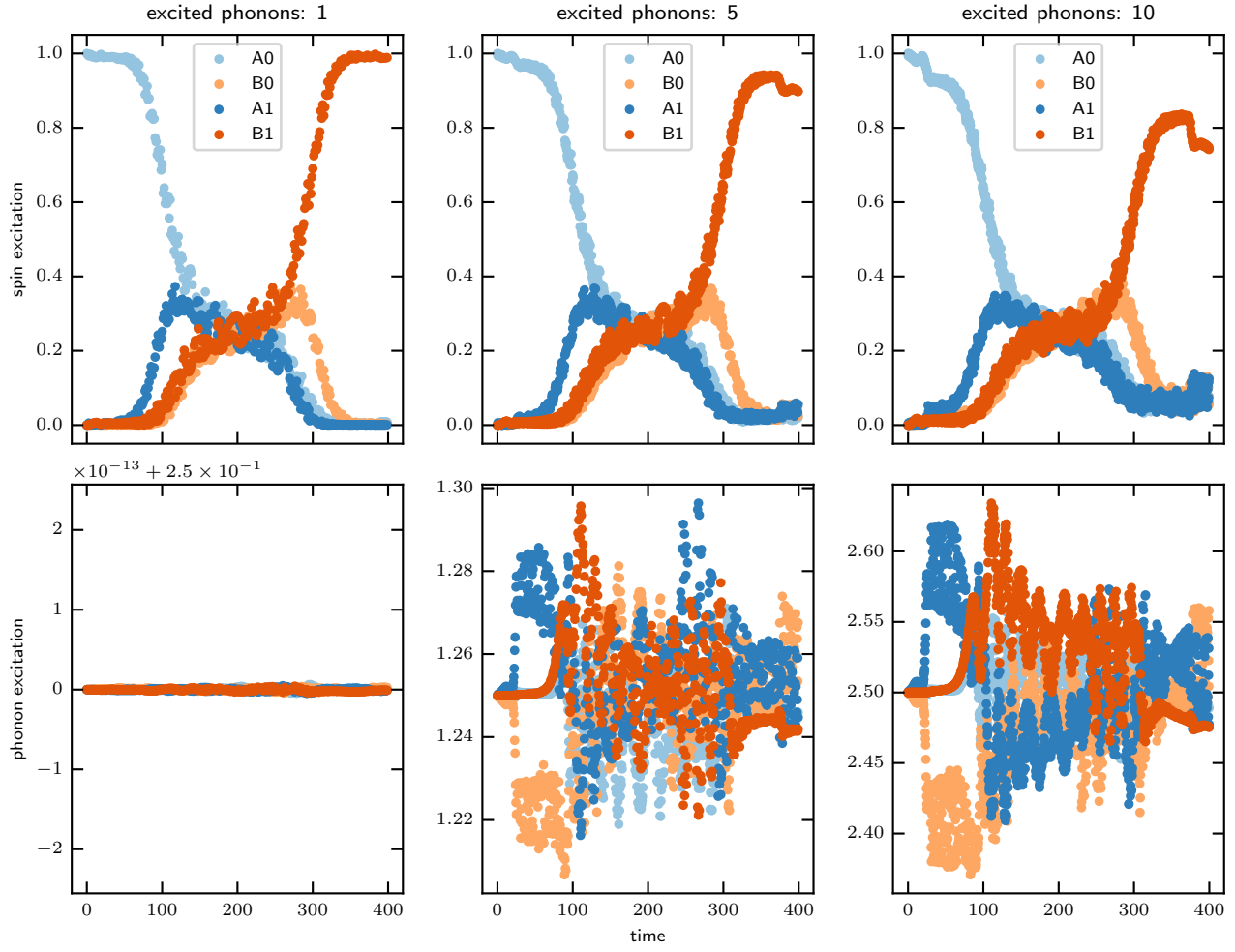
Figure 16: Rice-Mele scheme.
