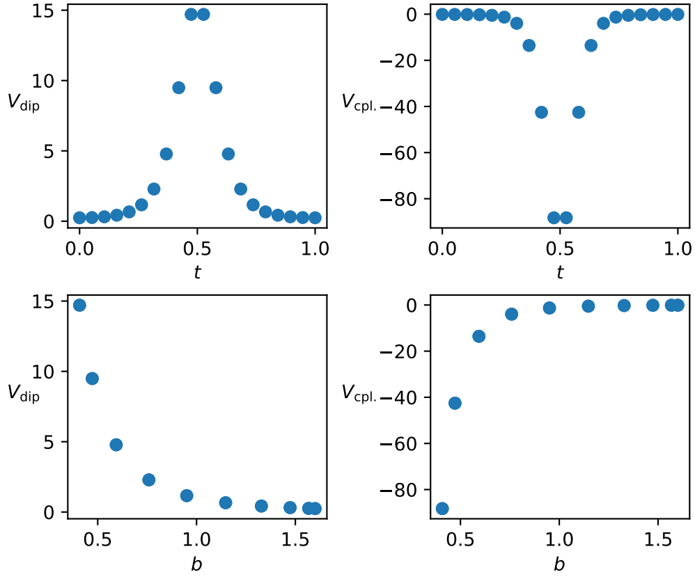
Figure 15: Interaction strengths during Rice-Mele scheme.
