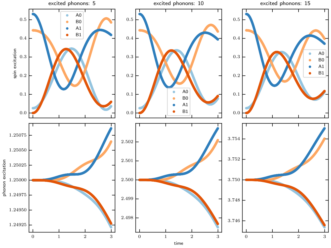
Figure 12: Evolution with full Hamiltonian ratio spin only: coupling 10:1.
