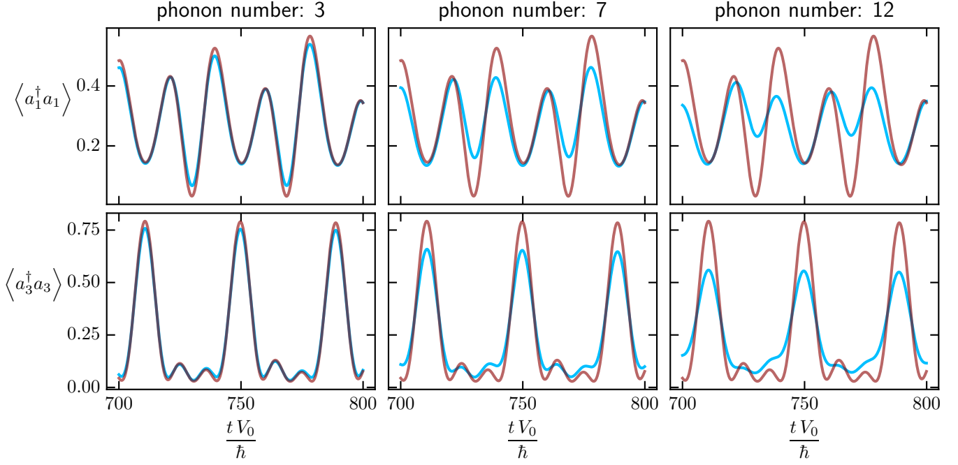
Figure 8: Comparison of free evolution with and without phonons. The difference in spin excitation probability between the free evolution with and without phonons is shown for a chain of length N = 4 . As initial conditions I chose a quadratically decaying excitation profile from the right edge and parameters b = 1.2r_0 , h = 0.4r_0 , a = 3r_0 . The red line shows the trajectory for the case without motional degrees of freedom and the blue one the case with phonons present. For an atom with 12 motional excitations the mean displacement is of the order of 0.15 \mu\text{m} , which is already around the limit of the expansion to second order being accurate.
