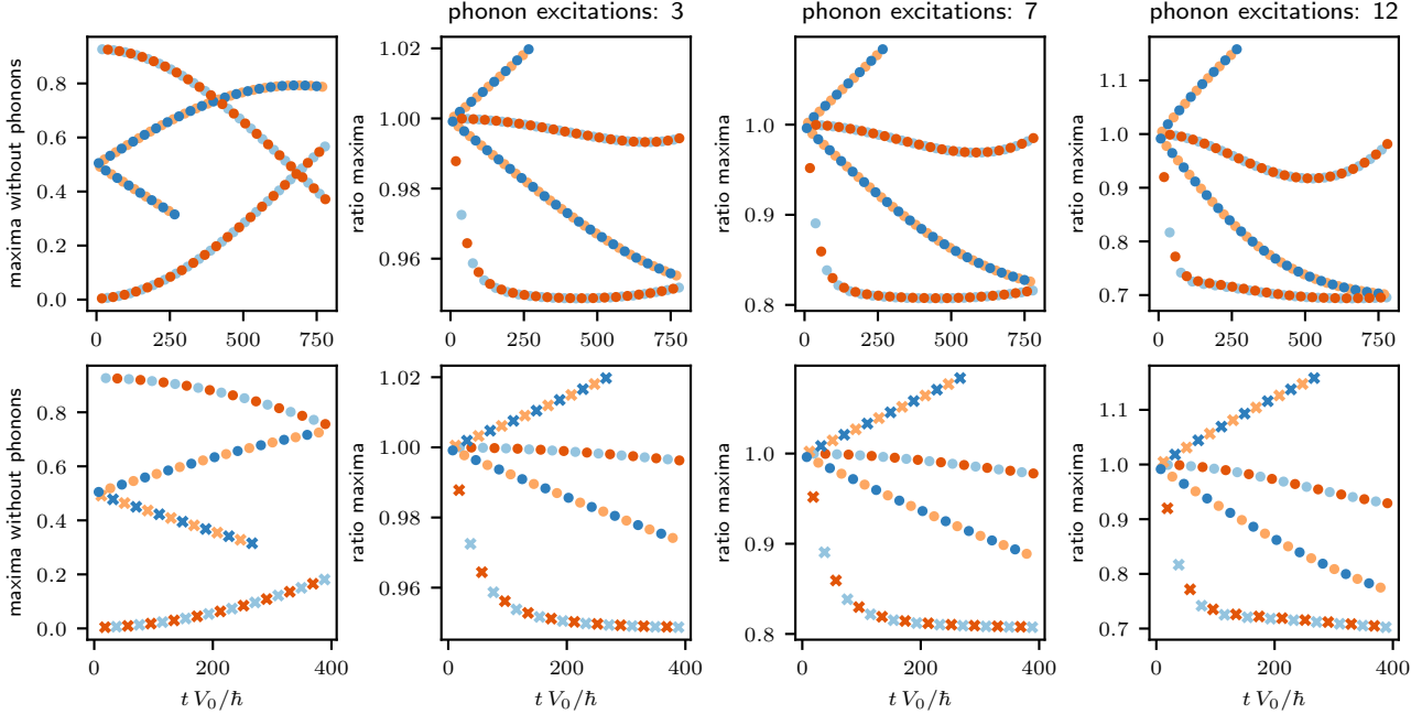
Figure 9: Comparison of the maxima of the free evolution with and without phonons. For the same parameters and initial conditions as in Fig. 8 the maxima of the spin excitation probability at the individual sites are compared for the free evolution with and without phonons.
