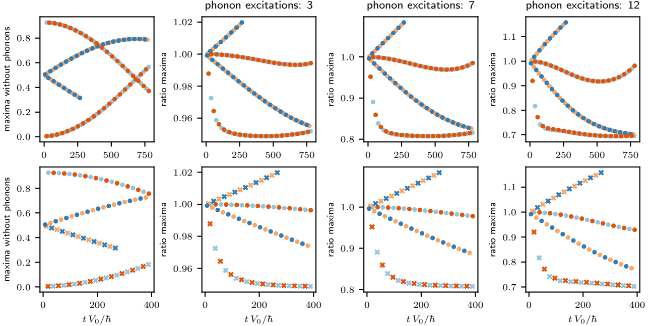
Figure 10: Comparison of the maxima of the free evolution with and without phonons. For the same parameters and initial conditions as in Fig. 9 the maxima of the spin excitation probability at the individual sites are compared for the free evolution with and without phonons.
