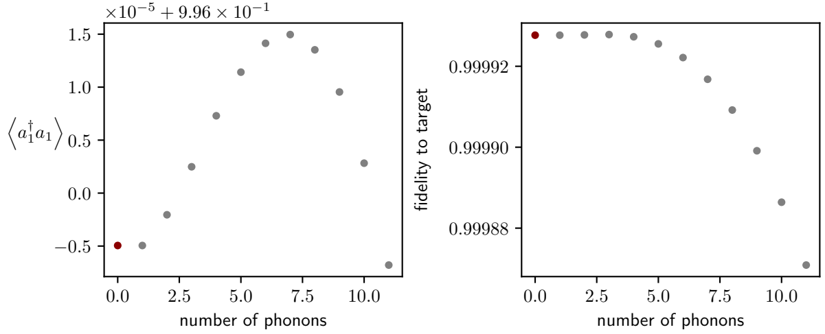
Figure 12: Transferred excitation in dependence of phonon number. I show the excitation probability at the left edge at the end of the cycle, when the system is initialized in an eigenstate of the pure spin Hamiltonian localized at the right edge. And parameters of the cycle are b = 1.8-1.2-1.8 r_0 , h = 0.4 r_0 , a = 3 r_0 , \Delta_{\max} = 0.4 V_0 .
