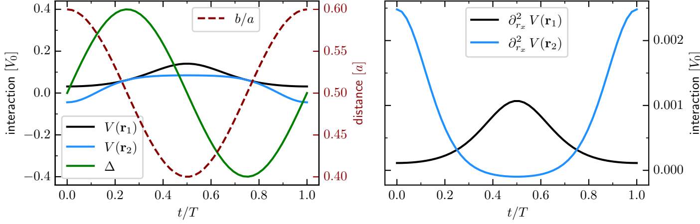
Figure 11: Rice-Mele scheme. Depicted is the course of the the decisive parameters during the Rice-Mele cycle, i.e. the axial distance between atoms in the unit cell b = 1.8-1.2-1.8 r_0 (the distance orthogonal to the chain axis is kept constant h = 0.4 r_0 as well as the distance inside a sublattice a = 3 r_0 ). The detuning takes it's maximal value at \Delta_{\max} = 0.4 V_0 .
