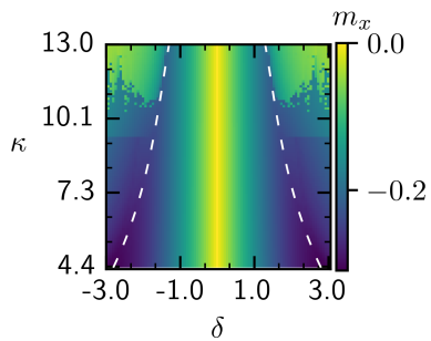
(a) m_x for \omega = 2.4
