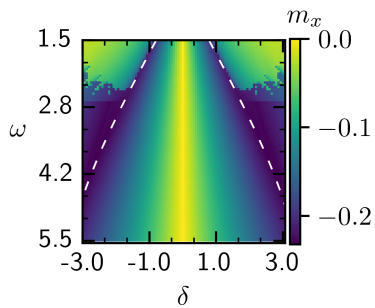
(b) m_x for \kappa = 11.3
