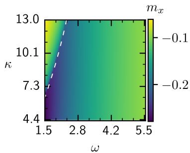
(c) m_x for \delta = -1.3
