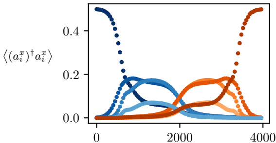
x-phonons
