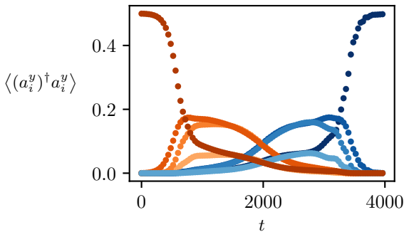
y-phonons
