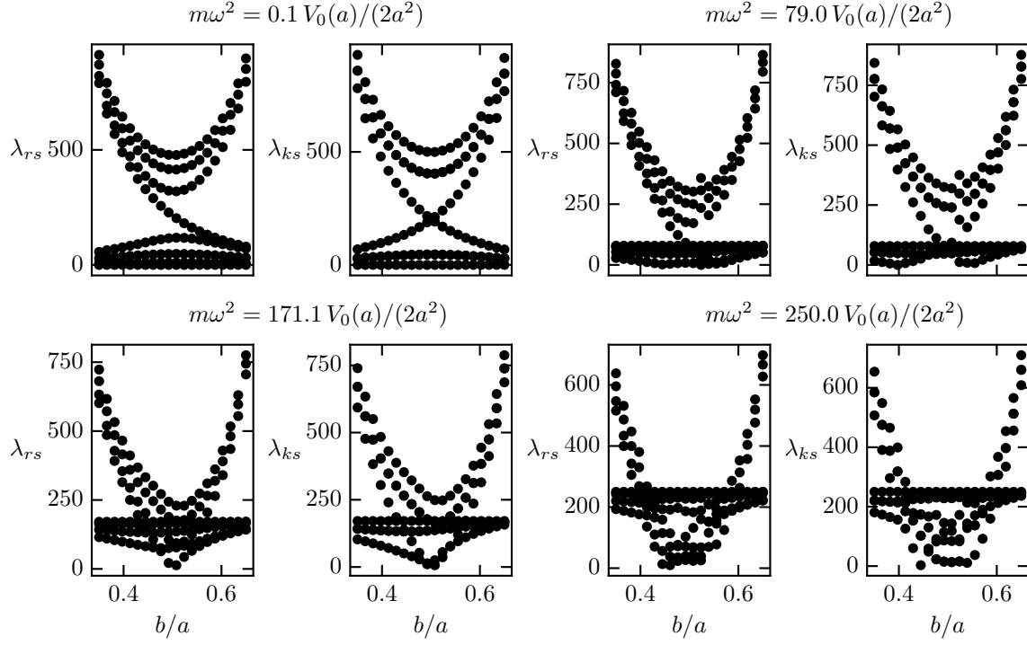
Figure 4: Spectrum of the U matrix in real and momentum space.
