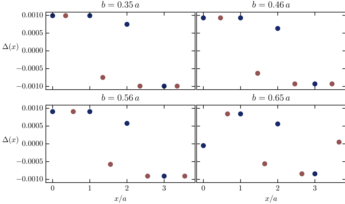
Figure 2.2: Trap center shift. For m\omega^2 = 10 V_{\max} the shift of the trap center for each site, that tunes the linear order to zero, is shown. The length of the chain is taken as 8 atoms.
