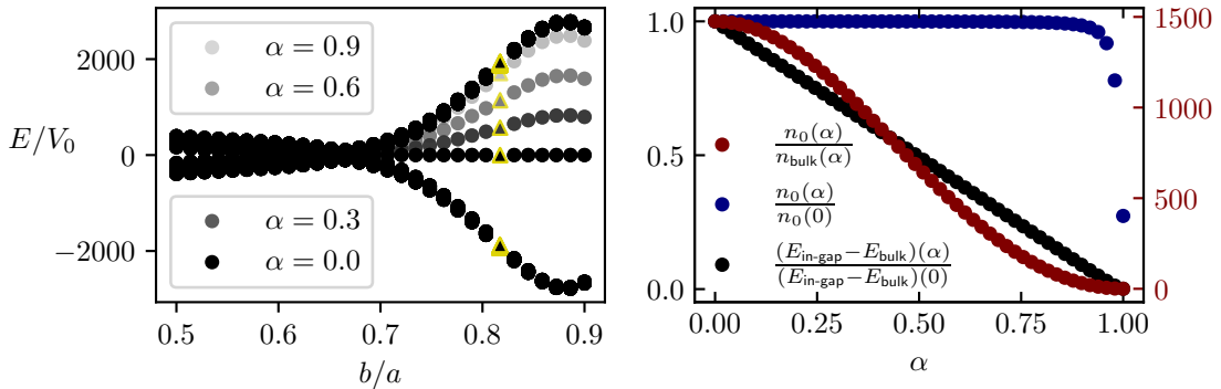
Figure 2.6: Edge occupation in dependence of onsite potential strength. The left panel shows the spectrum of H in dependence of the spacing between the atoms for different values of \alpha . Energies are given in units of V_0 = \hbar V(a)/(2m\omega a^2) . In the diagram, \alpha is an artificial factor with whom the diagonal of matrix H is multiplied, in order to show how this term pulls the in-gap modes into the bulk. For the highlighted b -values the left panel shows how the edge occupation degrades with increasing \alpha .
