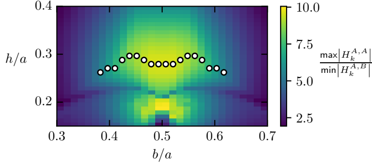
Figure 2.7: Optimal ratio between maximum of H_k^{A,A} and minimum of H_k^{A,B} . The ratio is computed taking into account nearest neighbor interactions for H_k^{A,B} and next to nearest neighbor interactions for H_k^{A,A} . The circles depict the 1D cross section for which the spectrum and the edge occupation is considered in Fig. 2.8.
