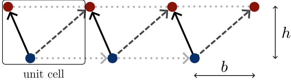
Figure 2.5: Zik-zak chain. Interactions up to next nearest neighbors are presented. The two sublattices A and B are depicted in colors red and blue respectively.
