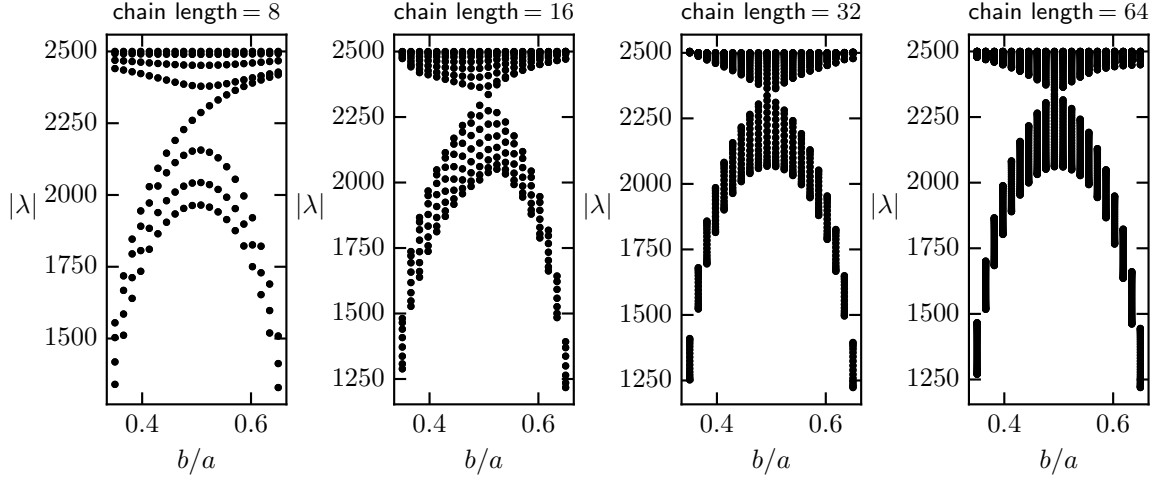
Figure 2.4: Positive spectrum of BdG Hamiltonian for different atom numbers.
