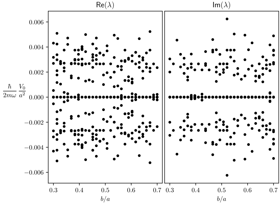
Figure 3: BdG spectrum for lattice size 80
