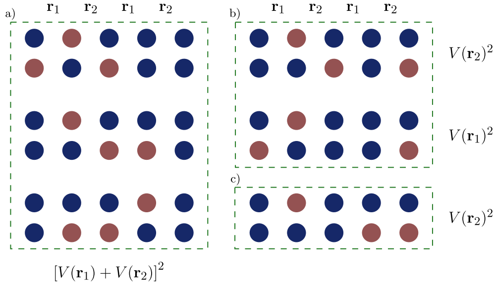
Figure 10: Coupling schemes. There are different ways double excited states couple to the single excited ones. The top row always depicts a state of the single, while the bottom row depicts a state of the double excited subspace. Generally configurations of two different subspaces are coupled to each other, when for two neighboring atoms one configuration has the inverted excitation scheme with respect to the other. I assign them to three categories. The first category is depicted in a). It couples two neighboring atoms twice. In the picture all possible cases are shown. For b) only two atoms couple two each other. Here the coupling takes place at a pair of |e\rangle and |g\rangle in both configurations. If the excitation in the single excitation subspace is at position 2 < i < N - 1 , there are N - 4 different states in the double excited subspace that contribute a term V(r_1)^2 and the same number for V(r_2)^2 . Category c) couples two unexcited sites in the single excitations subspace to two excited sites in the double excited subspace. For this case there are N/2 - 2 states that contribute V(r_1)^2 and N/2 - 2 states that contribute V(r_2)^2 , if the single excited state is excited at atom 2 < i < N - 1 .
