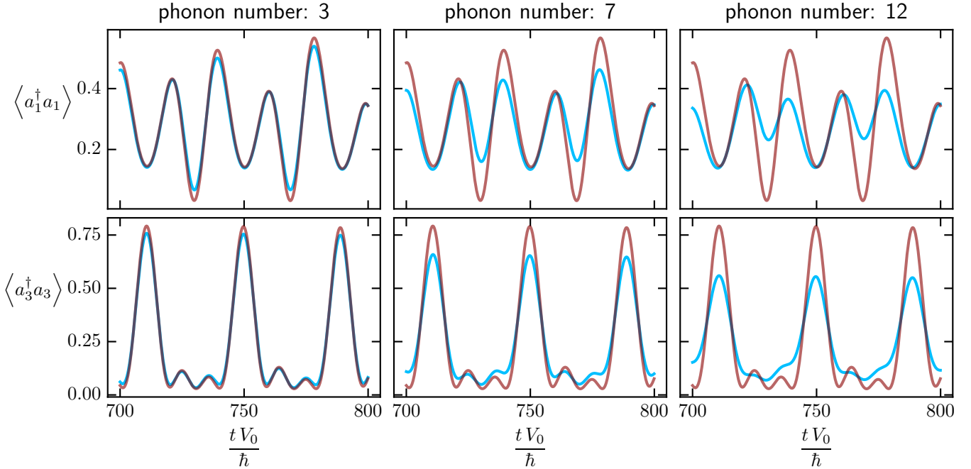
Figure 13: Comparison of free evolution with and without phonons. The difference in spin excitation probability between the free evolution with and without phonons is shown for a chain of length N = 4 . As initial conditions I chose a quadratically decaying excitation profile from the right edge and parameters b = 1.2r_0 , h = 0.4r_0 , a = 3r_0 . The red line shows the trajectory for the case without motional degrees of freedom and the blue one the case with phonons present. For an atom with 12 motional excitations the mean displacement is of the order of 0.15 \mu\text{m} , which is already around the limit of the expansion to second order being accurate.
