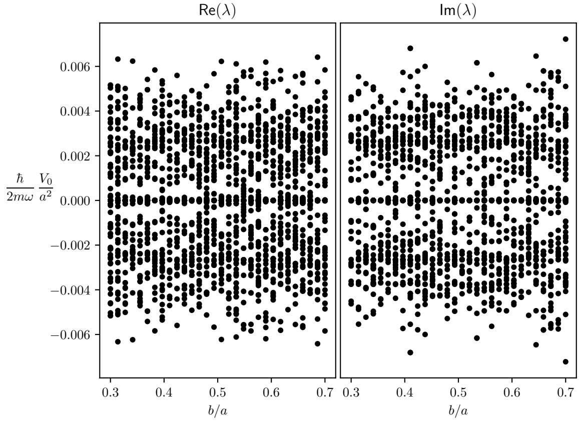
Figure 4: BdG spectrum for lattice size 800
