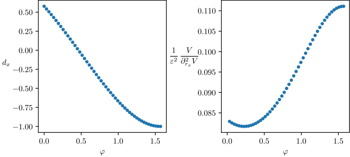
Figure 11: Dipole orientation and ratio of interactions. For all angles \sin \varphi := h/r one can find a dipole orientation, shown in the left panel, such that the first order term in the expansion of the interaction vanishes. The ratio between zeroth order and second order term is shown in the right panel.
