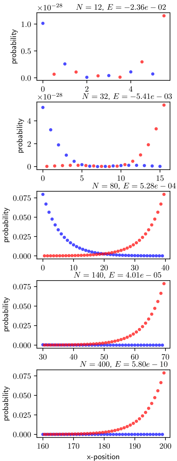
phonon direction x
