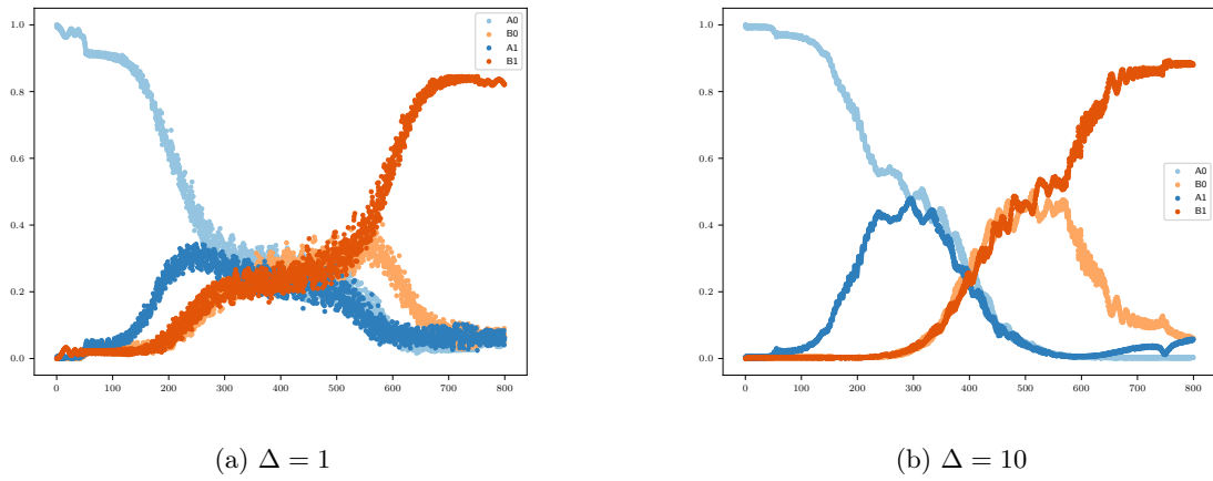
Figure 20: longer time evolution for phonon number 10.
