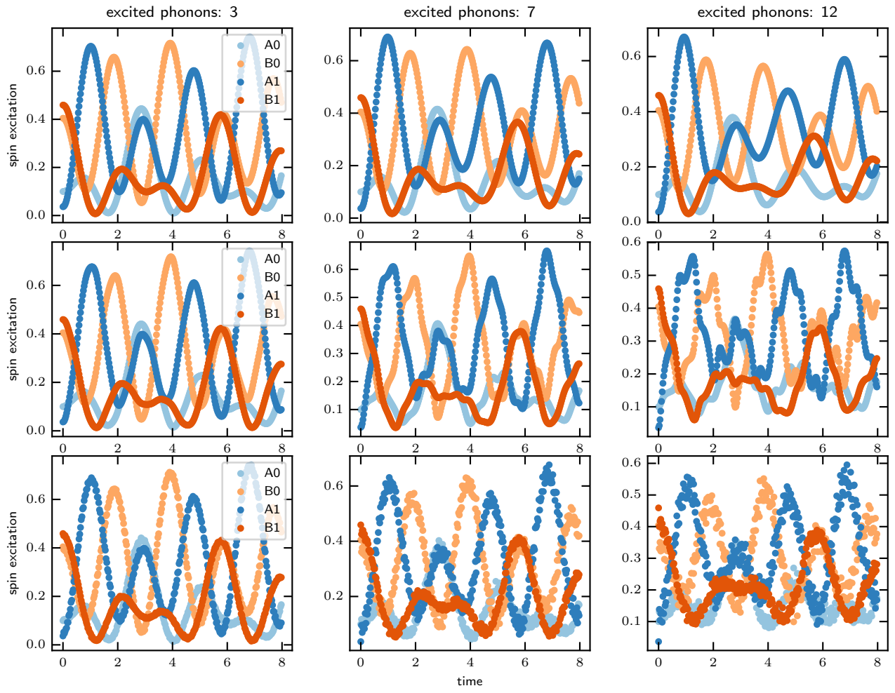
Figure 13: Summary spin evolution
