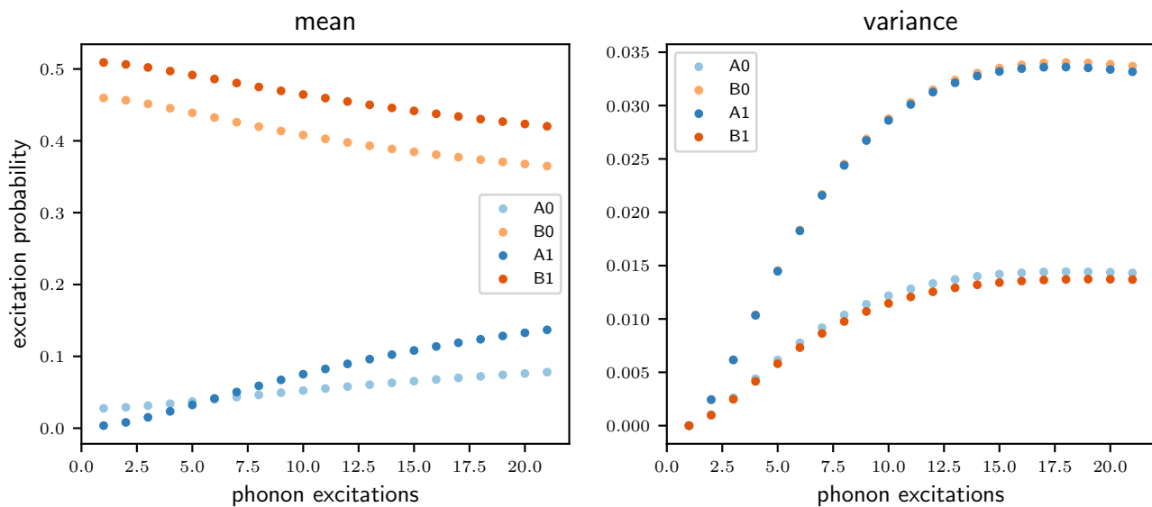
Figure 17: spin-phonon coupling only.
