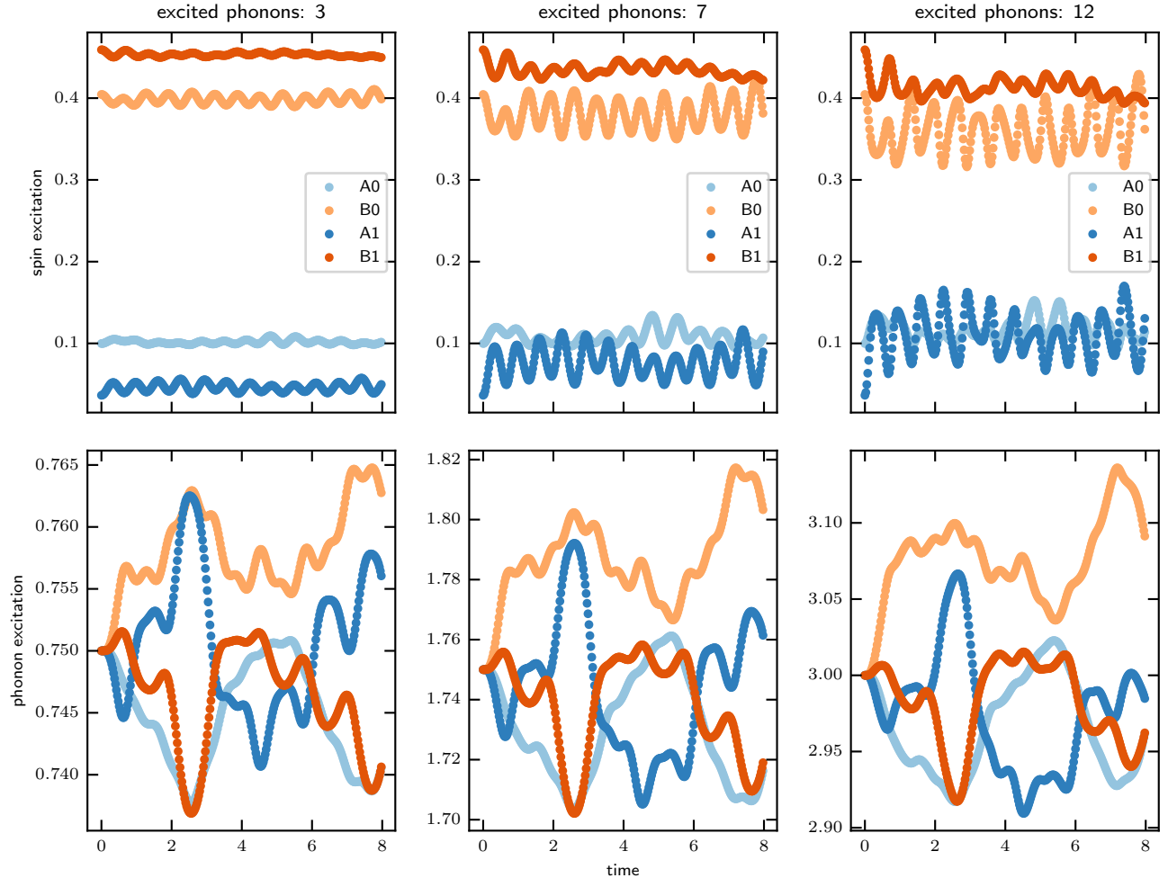
Figure 12: Evolution with only spin-phonon coupling term.
