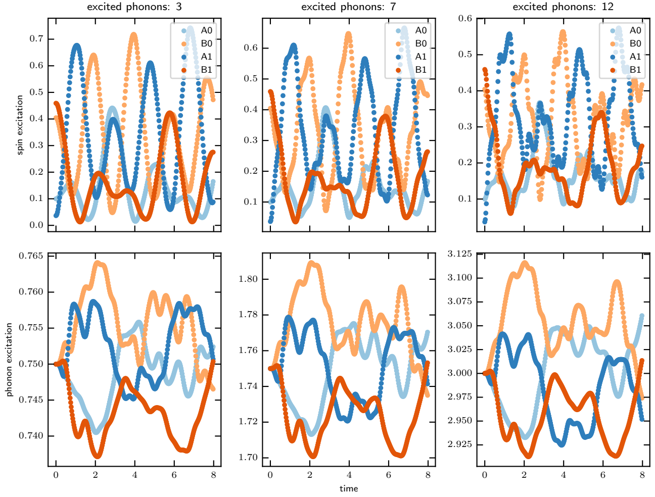
Figure 15: Evolution with full Hamiltonian ratio spin only: coupling 1:1.
