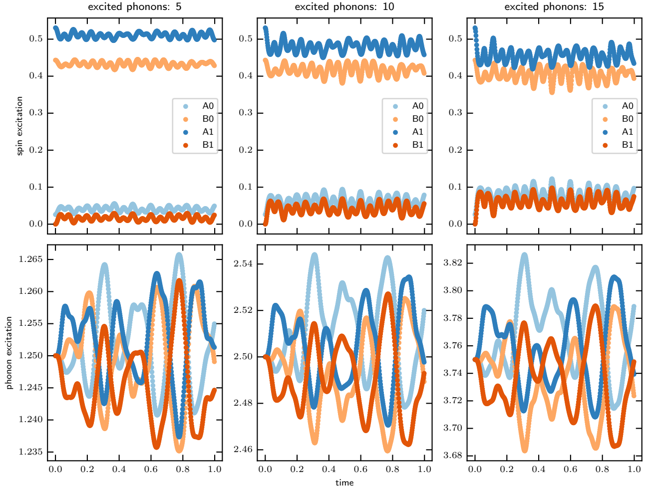
Figure 11: Evolution with only spin-phonon coupling term.
