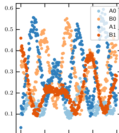
excited phonons: 12
