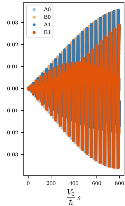
excited phonons: 3
