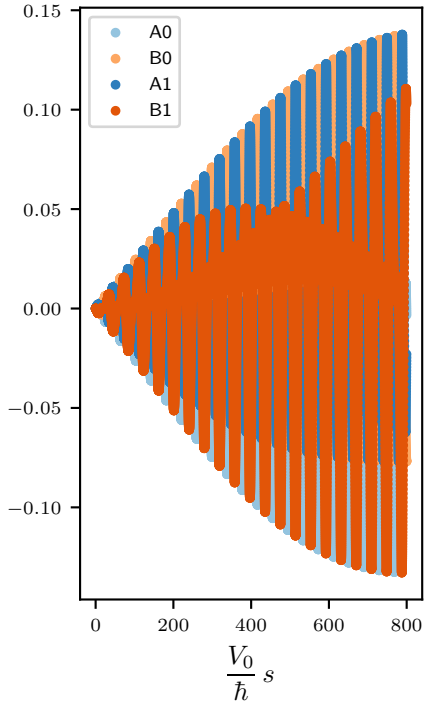
excited phonons: 7
