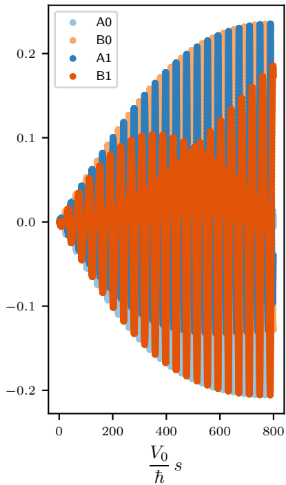
excited phonons: 12
