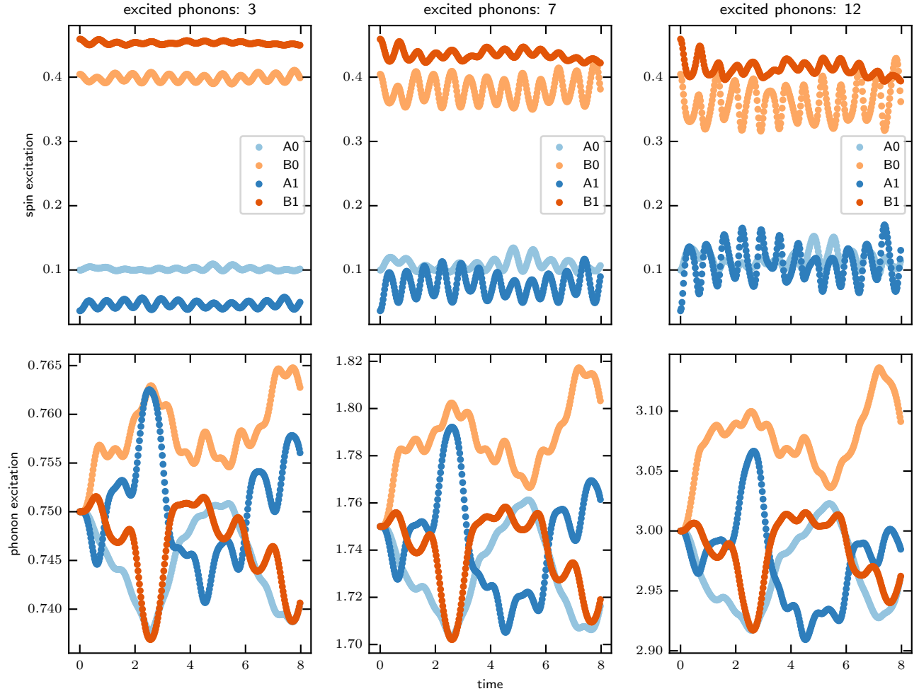
Figure 26: Evolution with only spin-phonon coupling term.
