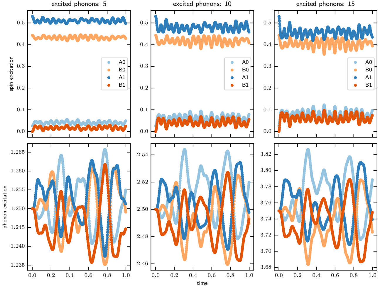
Figure 25: Evolution with only spin-phonon coupling term.
