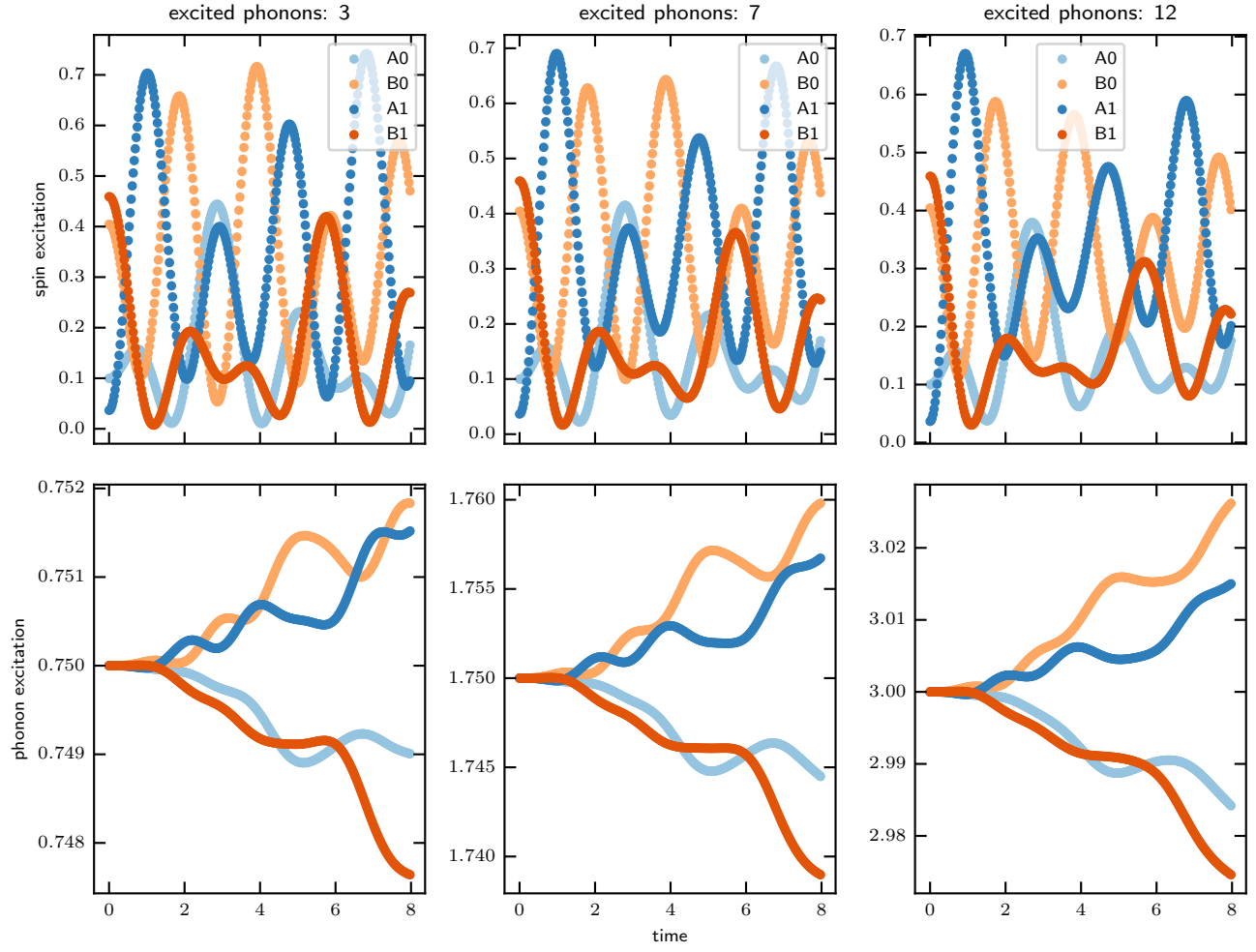
Figure 28: Evolution with full Hamiltonian ratio spin only: coupling 10:1.
