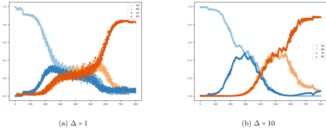
Figure 34: longer time evolution for phonon number 10.
