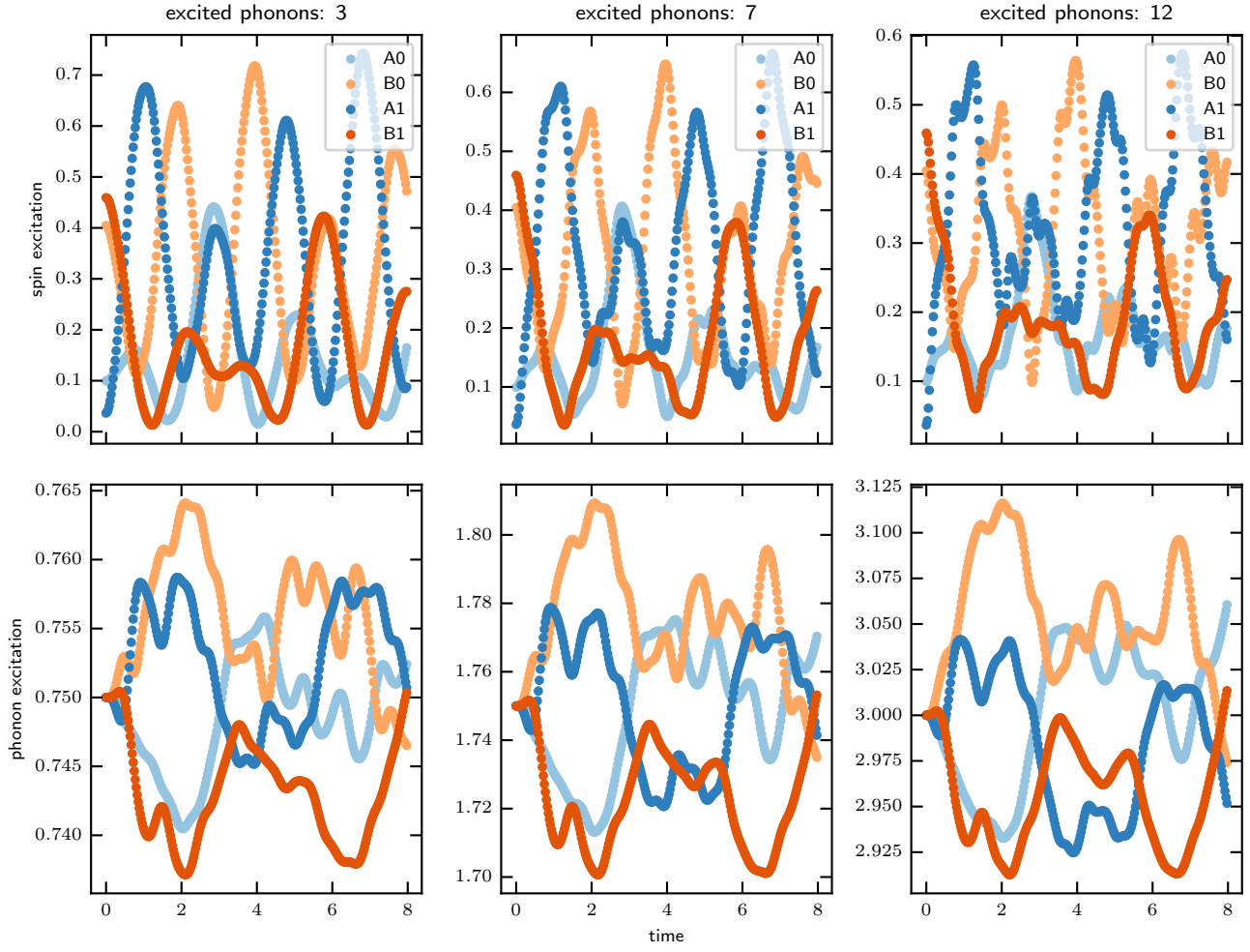
Figure 29: Evolution with full Hamiltonian ratio spin only: coupling 1:1.
