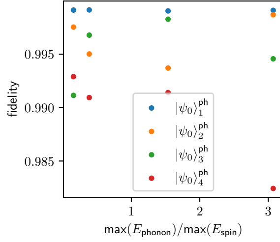
Figure 23: Fidelity in dependence of phonon interaction strength. For the 4 initial phonon configurations introduced in Fig. 22 (the labeling runs from top to bottom) different ratios of spin dipole interactions to phonon interactions are chosen. The fidelity between the final and target state is shown in dependence of interaction ratio and initial phonon state.
