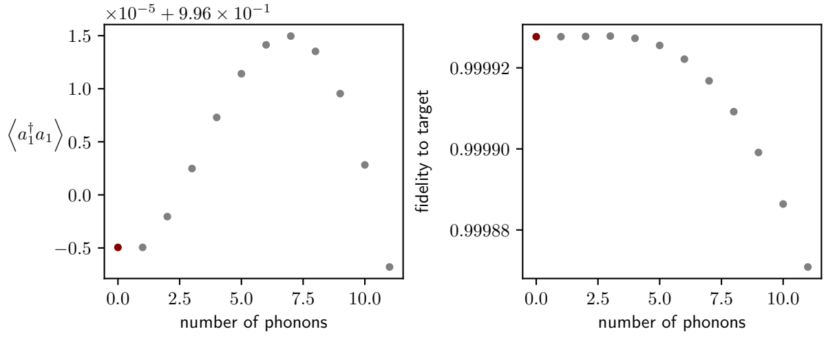
Figure 19: Transferred excitation in dependence of phonon number. I show the excitation probability at the left edge at the end of the cycle, when the system is initialized in an eigenstate of the pure spin Hamiltonian localized at the right edge. And parameters of the cycle are b = 1.8 - 1.2 - 1.8 r_0 , h = 0.4 r_0 , a = 3 r_0 , \Delta_{\max} = 0.4 V_0 .
