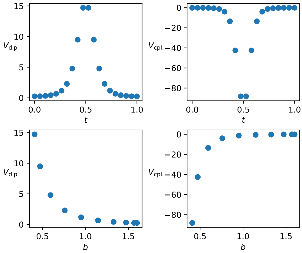
Figure 32: Interaction strengths during Rice-Mele scheme.
