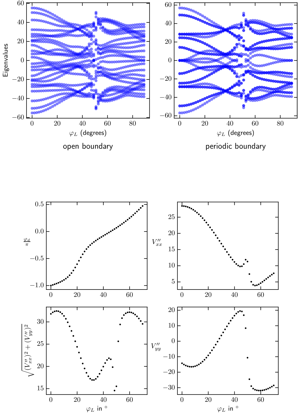
Figure 12: In this configuration with equal spacing between the atoms no topological states occur.
