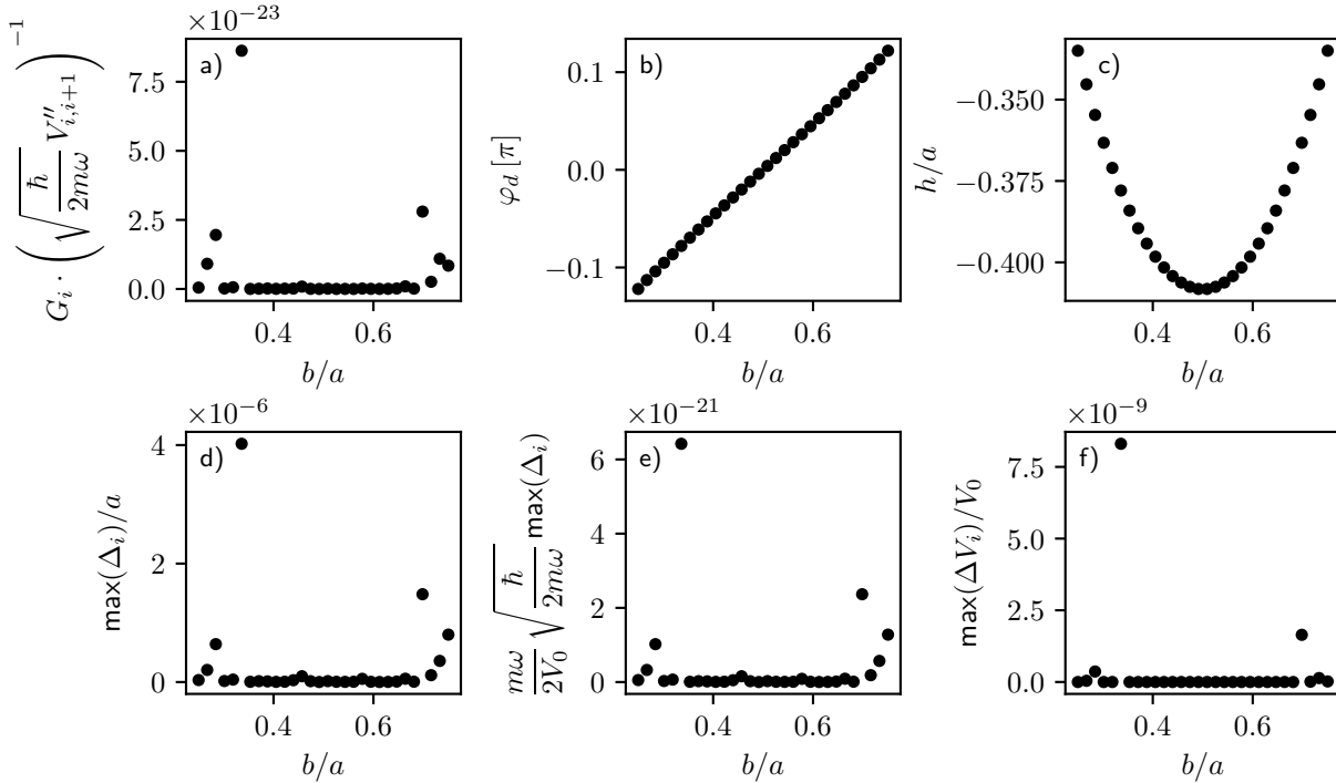
Figure 15: Parameters for negligible first order.
