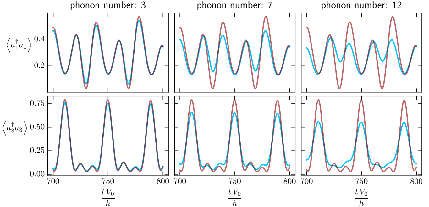
Figure 16: Comparison of free evolution with and without phonons. The difference in spin excitation probability between the free evolution with and without phonons is shown for a chain of length N = 4 . As initial conditions I chose a quadratically decaying excitation profile from the right edge and parameters b = 1.2r_0 , h = 0.4r_0 , a = 3r_0 . The red line shows the trajectory for the case without motional degrees of freedom and the blue one the case with phonons present. For an atom with 12 motional excitations the mean displacement is of the order of 0.15 \mu\text{m} , which is already around the limit of the expansion to second order being accurate.
