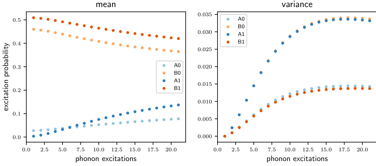
Figure 31: spin-phonon coupling only.
