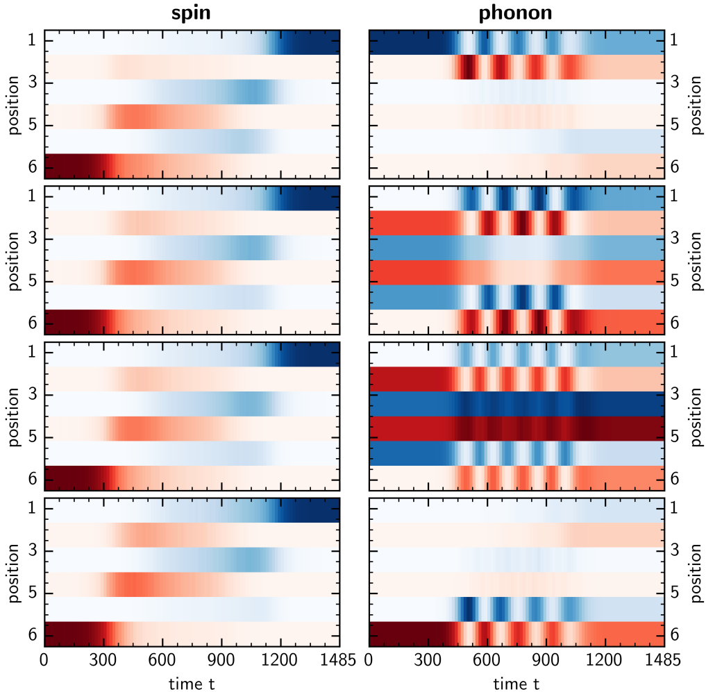
Figure 22: Spin transfer process. The time evolution of the spin and phonon degrees of freedom is depicted during the adiabatic transfer protocol. For the same transfer protocol the system was prepared in different initial phonon configurations, which stored one excitation in total.
