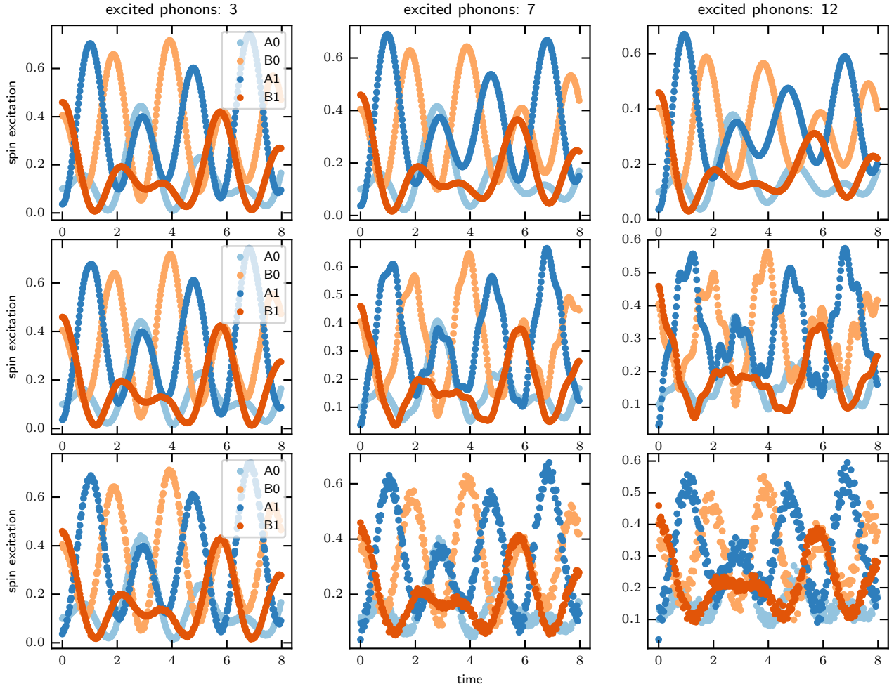
Figure 27: Summary spin evolution
