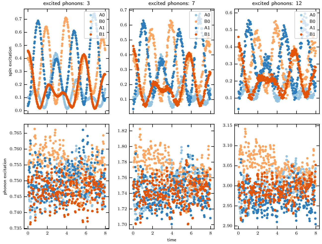
Figure 30: Evolution with full Hamiltonian ratio spin only: coupling 1:10.
