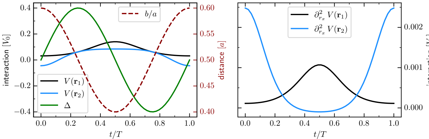
Figure 18: Rice-Mele scheme. Depicted is the course of the the decisive parameters during the Rice-Mele cycle, i.e. the axial distance between atoms in the unit cell b = 1.8 - 1.2 - 1.8 r_0 (the distance orthogonal to the chain axis is kept constant h = 0.4 r_0 as well as the distance inside a sublattice a = 3 r_0 ). The detuning takes it's maximal value at \Delta_{\max} = 0.4 V_0 .
