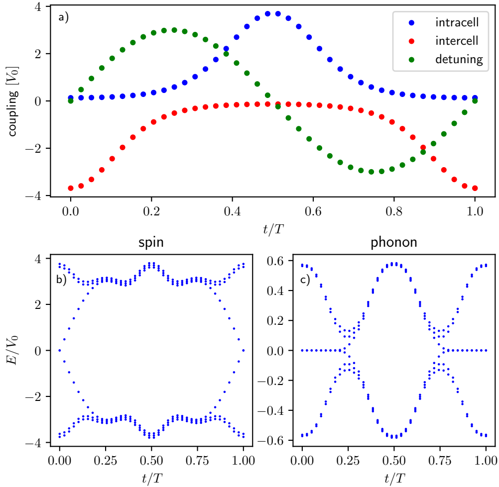
Figure 21: Spin transfer protocol. In a the course of the interaction during the transfer protocol is shown. b-c show the spectrum of the spin and phonon Hamiltonian respectively during the pump cycle each for one excitation in the respective degrees of freedom. For the spin Hamiltonian a pure dipole dipole interaction is used, where the dipole moments of the atoms are orientated in way that puts the interactions within the same sublattice to zero. This choice improves the accuracy of the nearest neighbor assumption. The phonon spectrum is received by the methods used in the previous chapters. It therefore depicts a scenario without spin degrees of freedom.
