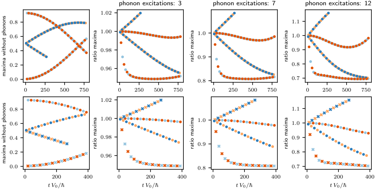
Figure 17: Comparison of the maxima of the free evolution with and without phonons. For the same parameters and initial conditions as in Fig. 16 the maxima of the spin excitation probability at the individual sites are compared for the free evolution with and without phonons.
