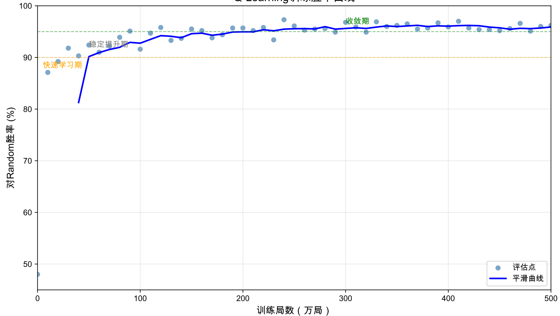
Q-Learning训练胜率曲线
