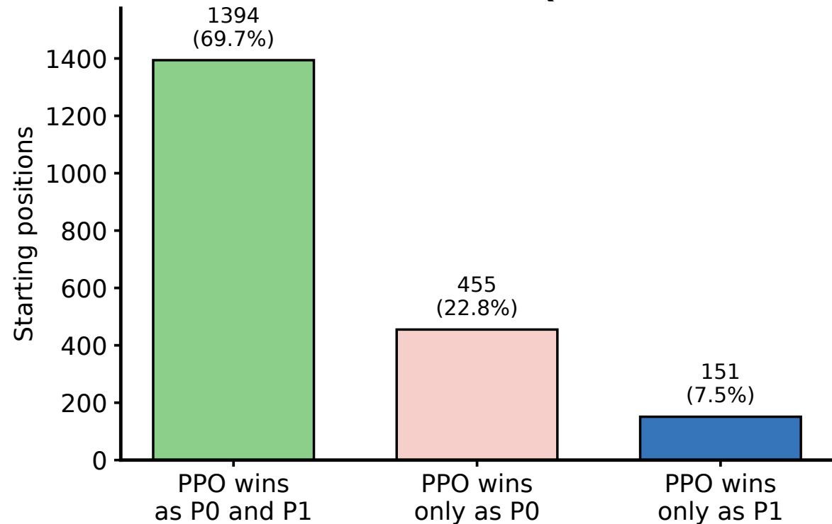
a Deterministic PPO vs Q-table
