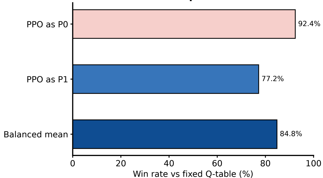
b Role-conditioned performance
