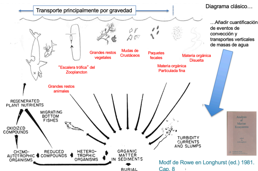
FIG. 5 Categories of possible sources of organic matter for deep-sea organisms
