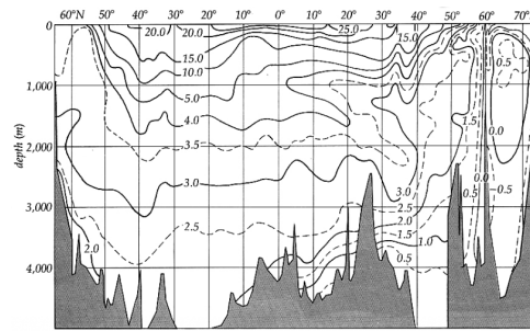
8.5 North-south temperature profile (in °C) of the Atlantic Ocean. The dark region represents a profile of the ocean floor, although the horizontal scale is compressed considerably; the vertical scale is considerably exaggerated.
