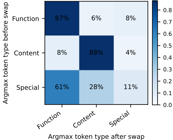
Changed-argmax transitions
