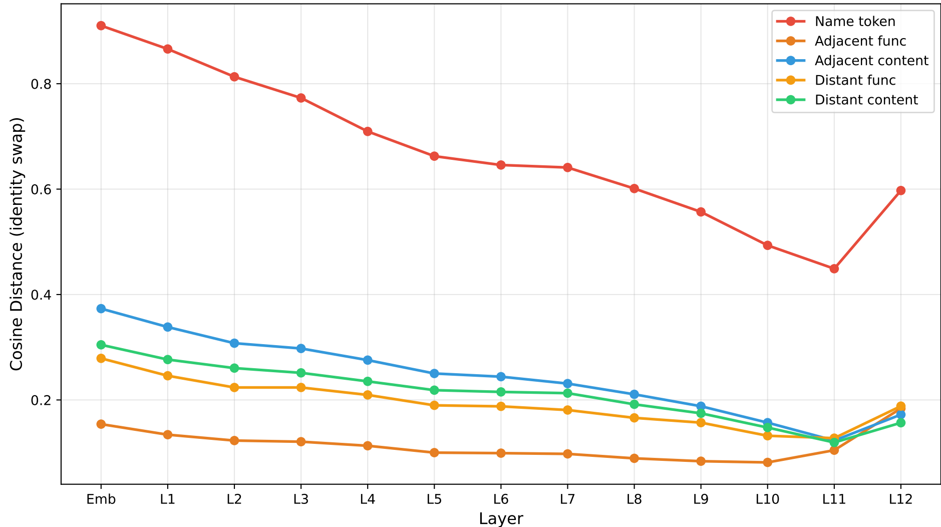
Representational Shift by Layer and Token Type
