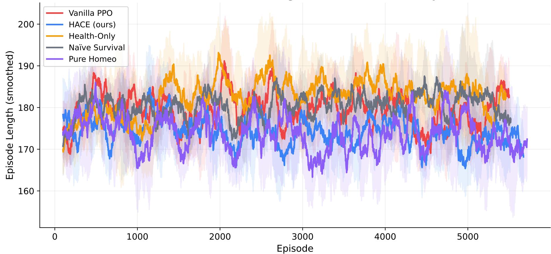
Survival Duration Learning Curves (Crafter, 1M Steps)
