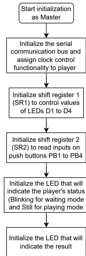
Subroutine to initialize as Master
