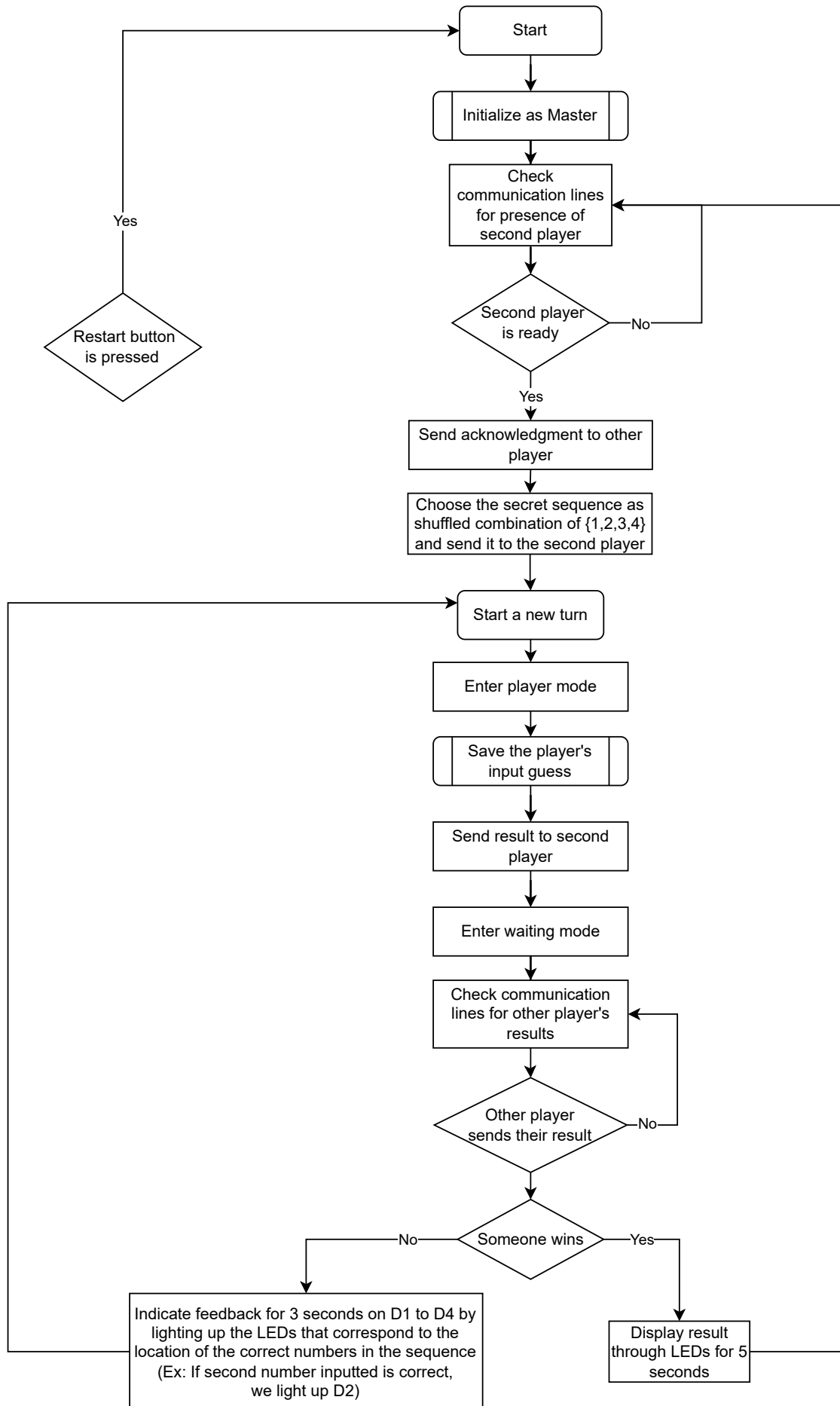
Player 1 Flow Chart
