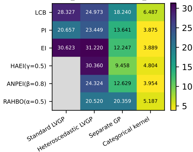
rastrigin_6d (final regret, n_rep=10)
