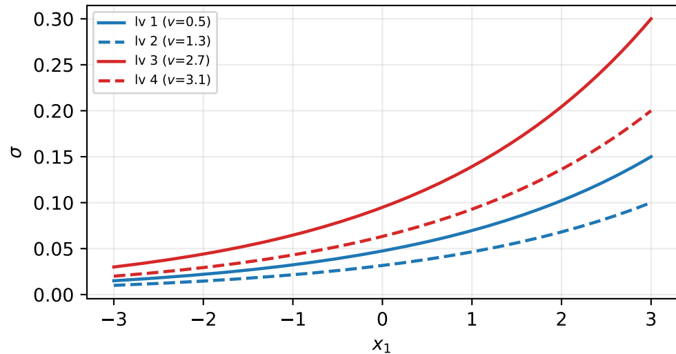
noise std: exponential ramp in x_1 (quiet at -3 , loud at +3 )
