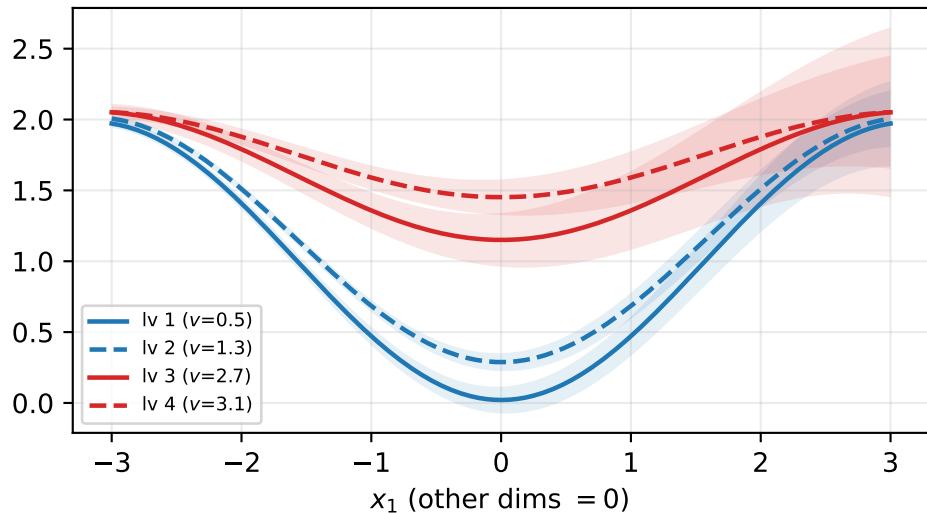
main-effect slice: true f per level ( \pm 2\sigma band)
