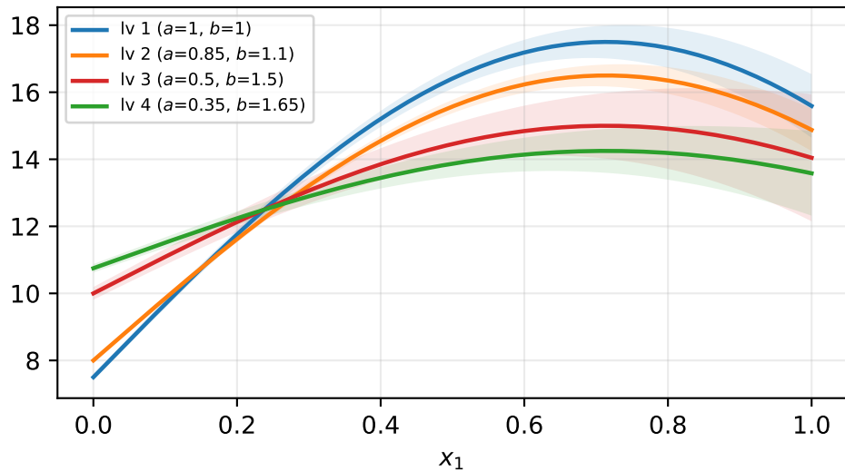
slice x_2 = 0.7 , others 0.5 (\pm 2\sigma \text{ band})
