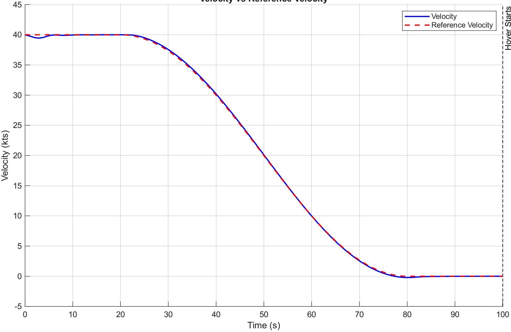
Velocity vs Reference Velocity
