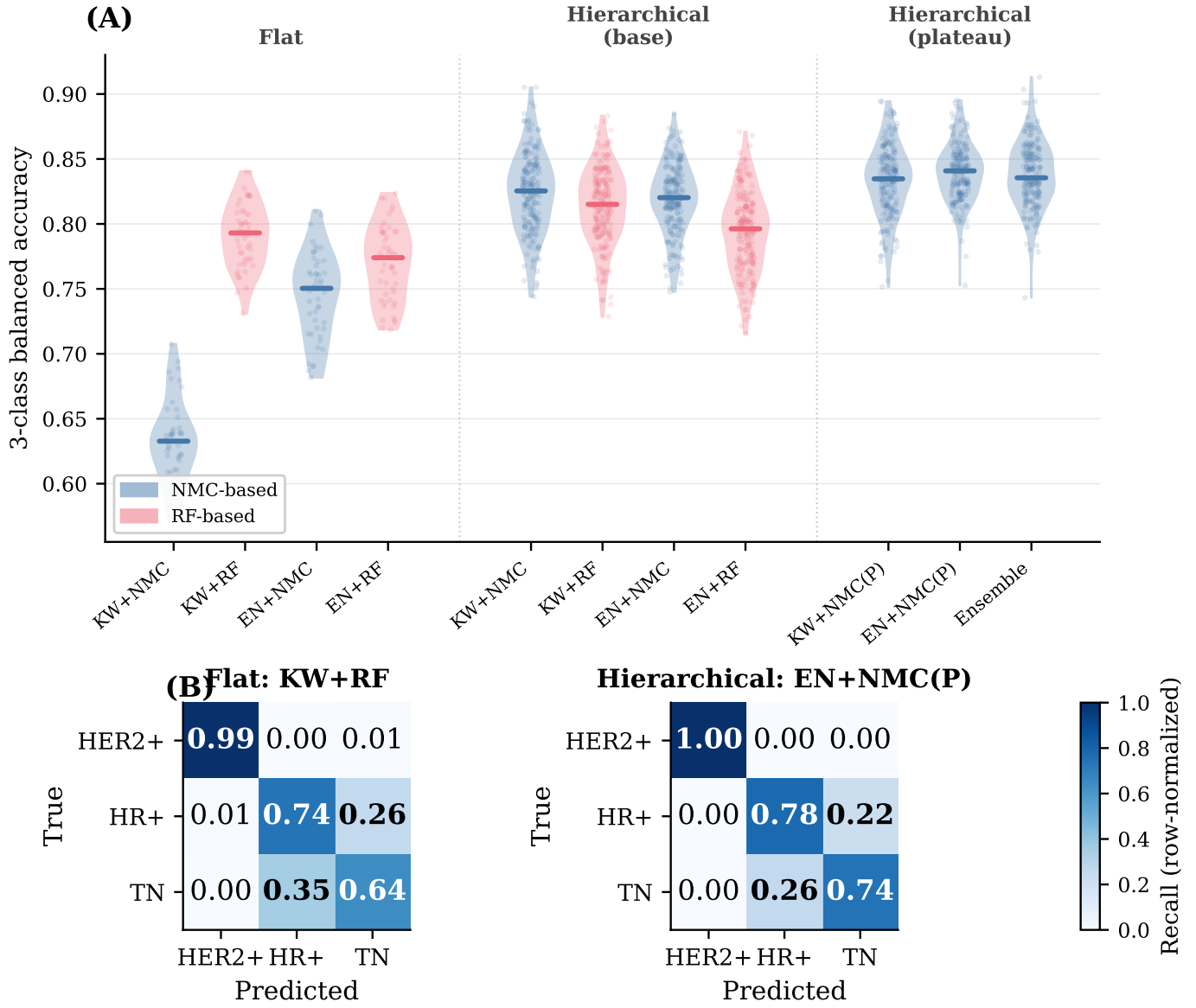
Figure 3: Model comparison. (A) BA distributions per pipeline (50 repeats flat, 200 hierarchical). All hierarchical variants outperform the best flat pipeline. (B) Confusion matrices for KW+RF (flat, left) and EN+NMC(P) (hierarchical, right), pooled over all outer folds.
