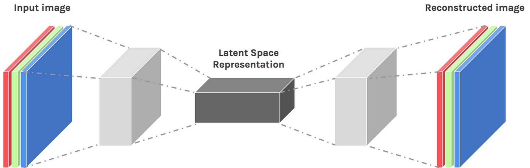
U-Net architecture
