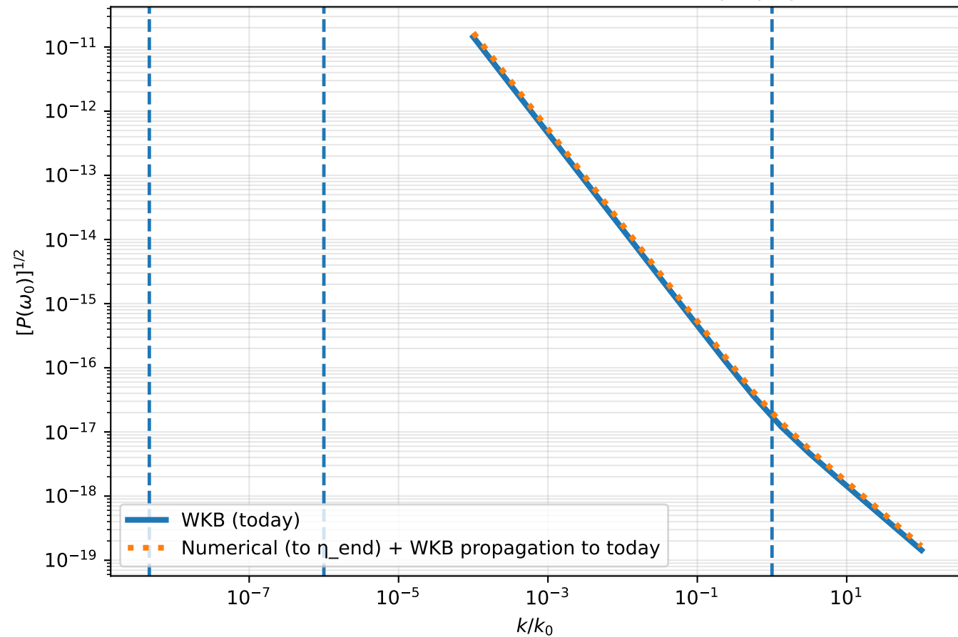
WKB vs numerical with consistent late-time propagation
