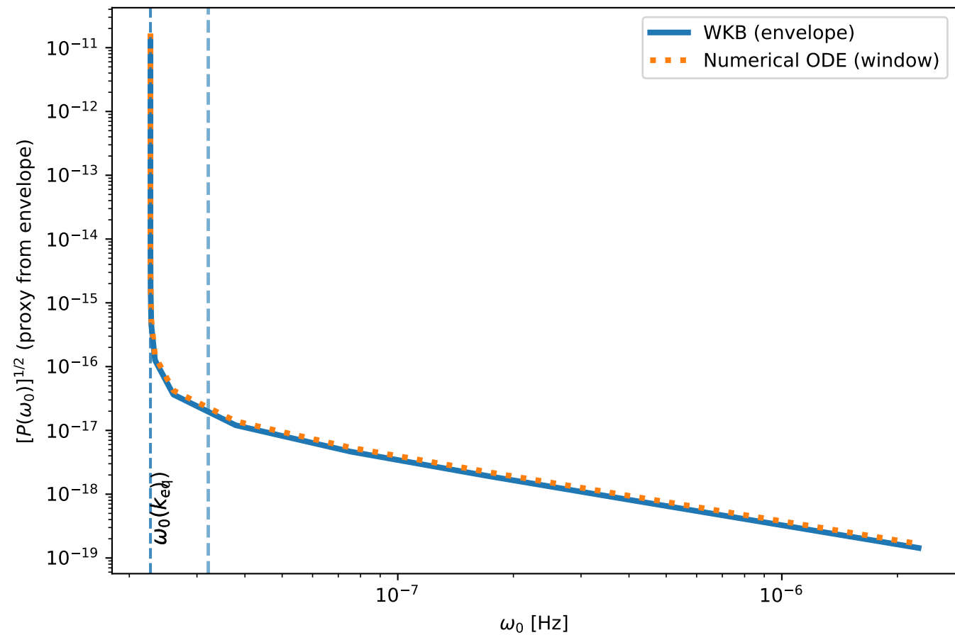
WKB vs numerical (window) mode amplitude vs \omega_0
