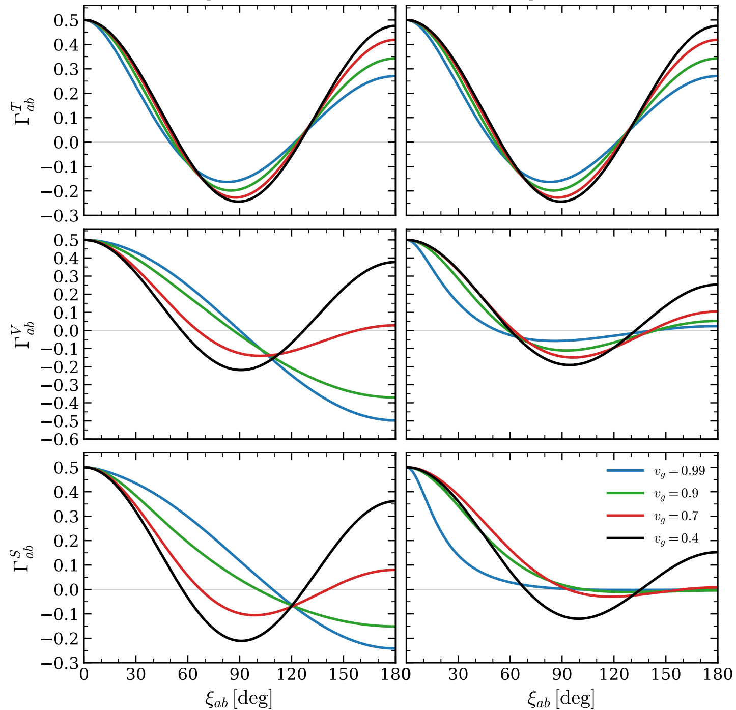
Liang-Trodden No pulsar terms
