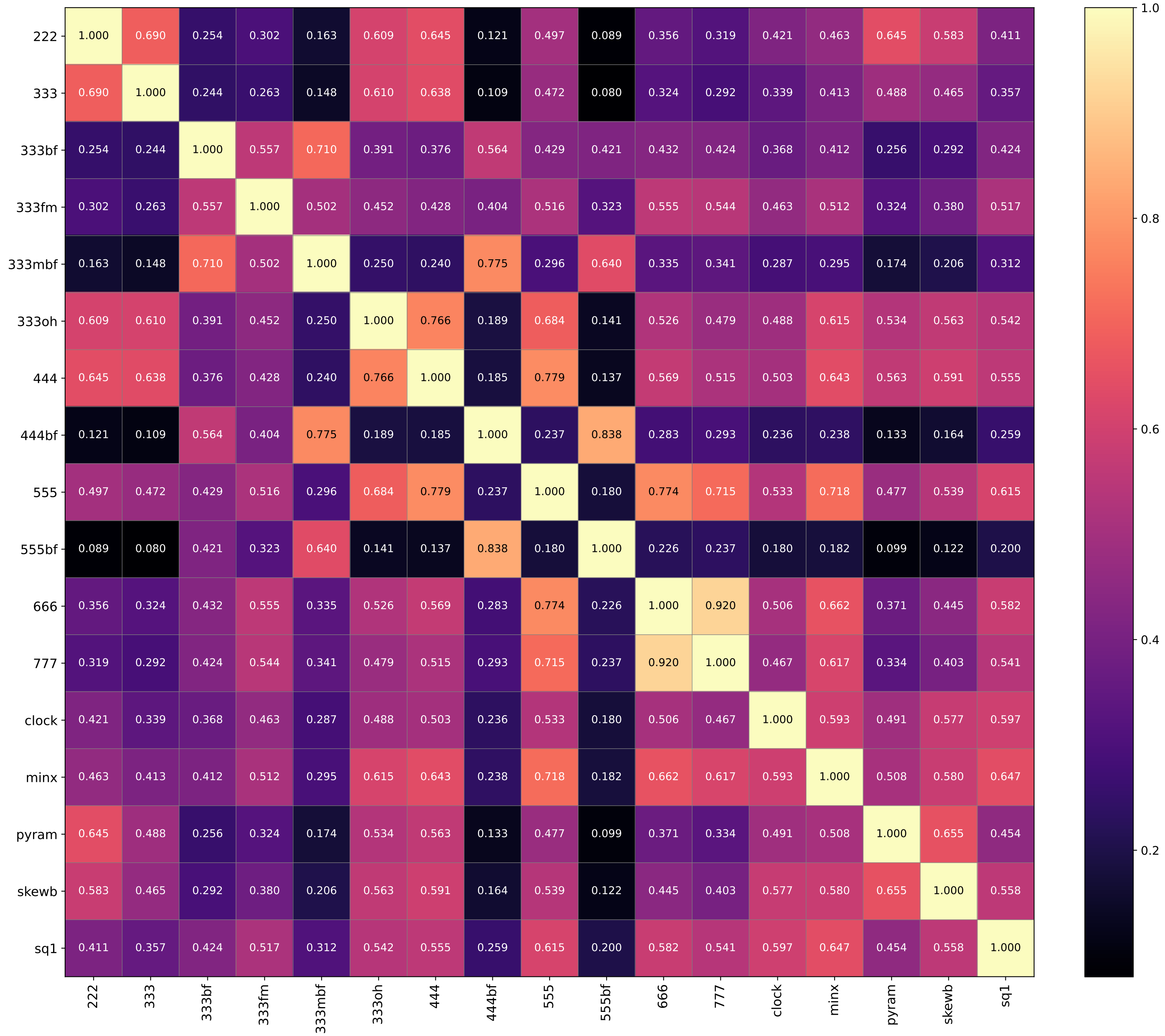
WCA Event Percentile Rank Correlation (n = 288288)
