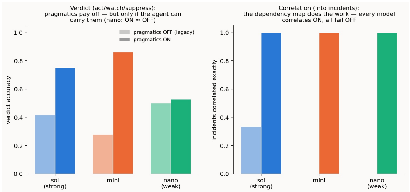
Figure 3. Left: verdict accuracy, pragmatics OFF (pale) vs ON (solid). The strong and mid agents gain sharply; the weak agent barely moves — ON ≈ OFF. Right: incidents correlated exactly. Every model correlates with the dependency map and fails without it.
