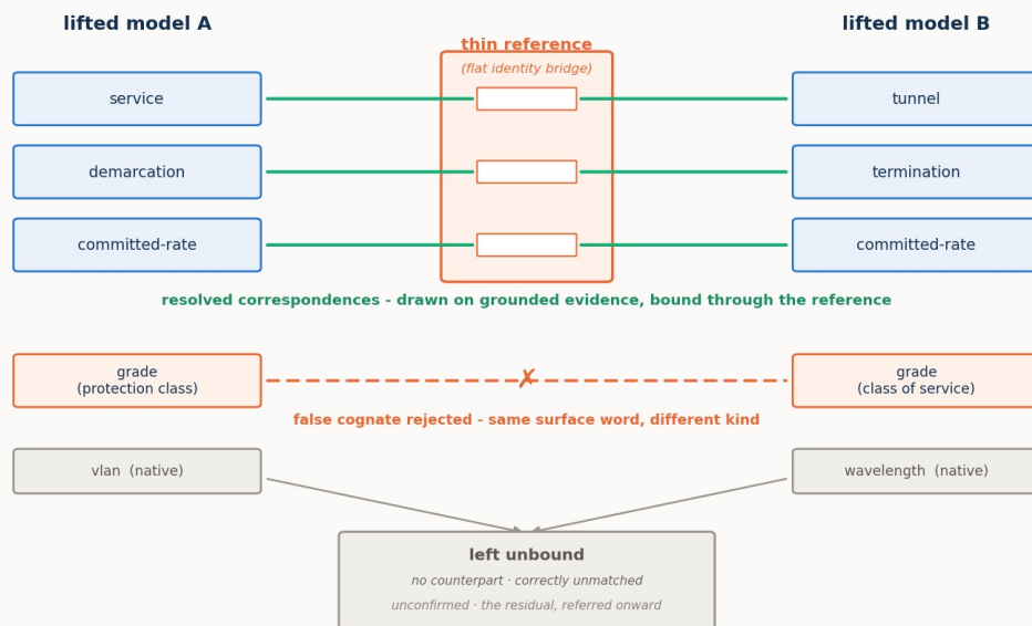
Figure 2. Reconciliation over two lifted models. Correspondences are drawn on grounded evidence and bound through a thin reference that anchors the shared common ground; a look-alike that shares only a surface word is rejected as a false cognate on its kind, attachment, and instances; a concept with no counterpart in the other model is correctly returned as unmatched, a resolved outcome, not a gap; and a correspondence the evidence cannot yet confirm is left in the residual, referred onward. The reference carries no meaning of its own; it works only by tying into the two grounded models it connects.
