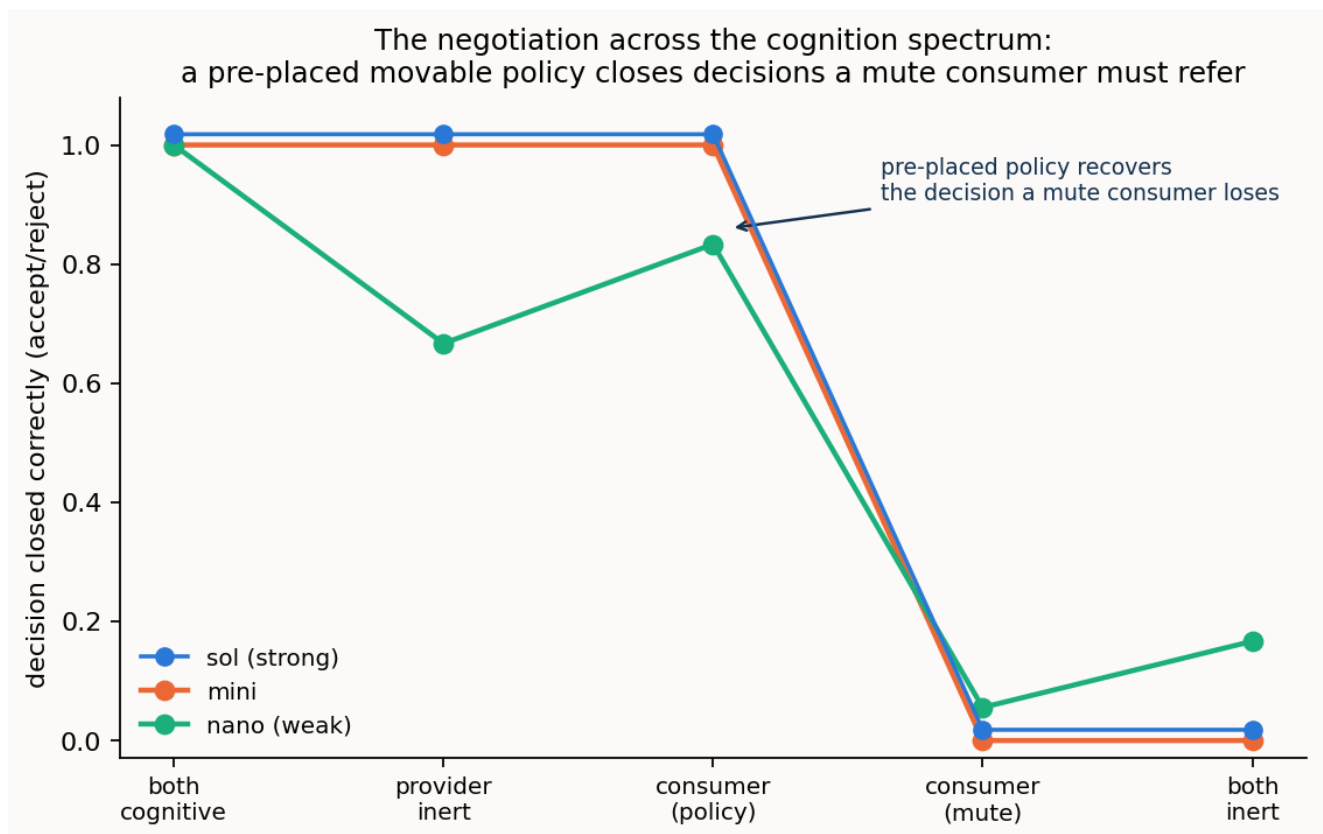
Figure 12 (setting 2). Decision accuracy across the cognition spectrum. It holds high while the customer's judgement is present (live, or pre-placed in a movable policy) and collapses to referral at consumer-mute and both-inert.
