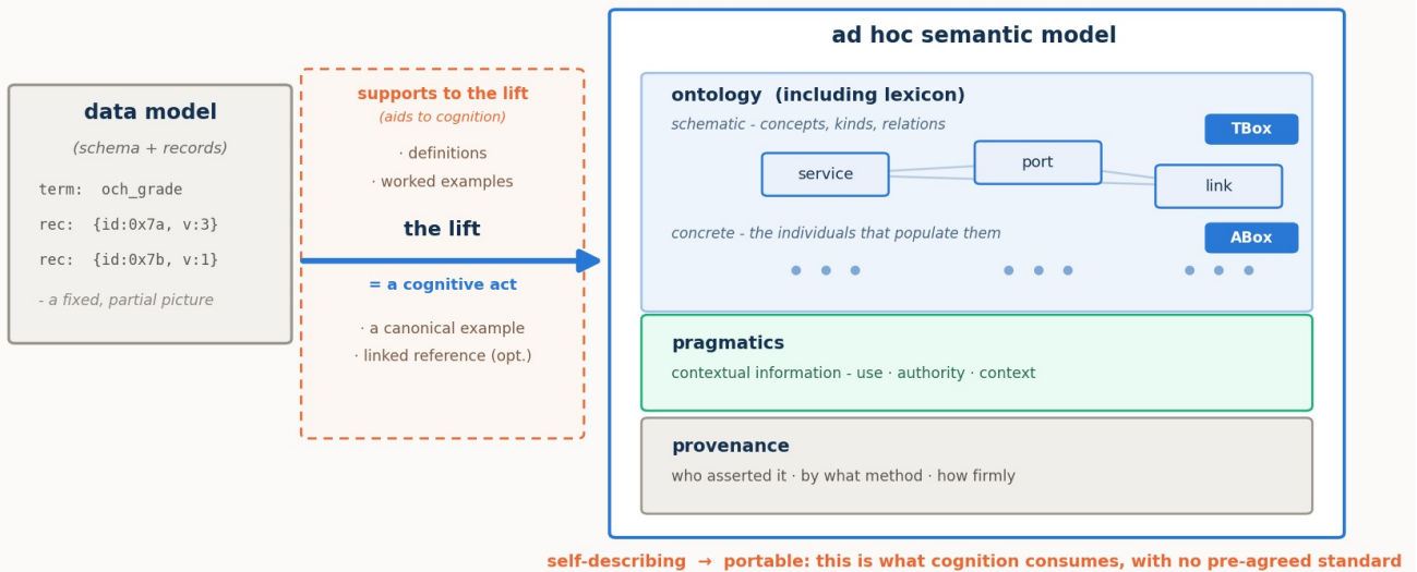
Figure 1. The lift. A data model (schema plus records) is a partial semantic picture, fixed by its format, with much of its meaning left implicit: in specifications, convention, and the engineers who built around it. The lift is a cognitive act, aided by a few supports (definitions, worked examples, a canonical example, an optional linked reference), that turns the data model into an ad hoc semantic model built from three parts: an ontology including its lexicon (a schematic layer of concepts, kinds and relations, the TBox, and the concrete instances that populate them, the ABox), pragmatics (use, authority, context), and provenance. Being self-describing, the result is portable: any cognitive consumer can pick it up and understand it, with no pre-agreed standard.
