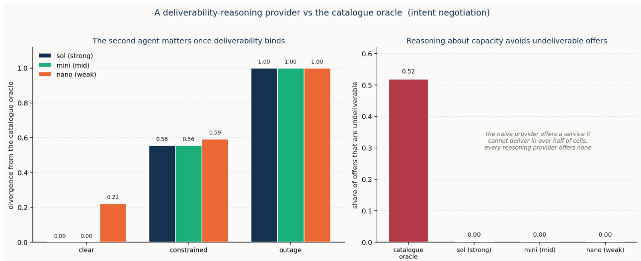
Figure 5.3. Left: the reasoning provider's divergence from the catalogue oracle by regime, per model — near zero while paths are clear (the §5.1 fixed-catalogue regime) and rising as paths saturate and the provider must counter-propose or decline. Right: the catalogue
