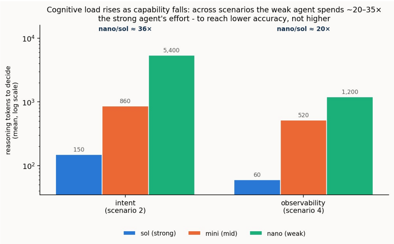
Figure 9. What you are looking at is the reasoning tokens (a model's hidden deliberation) each model spends to reach one such decision — one accept-or-reject of a degraded offer in the intent negotiation, or one
