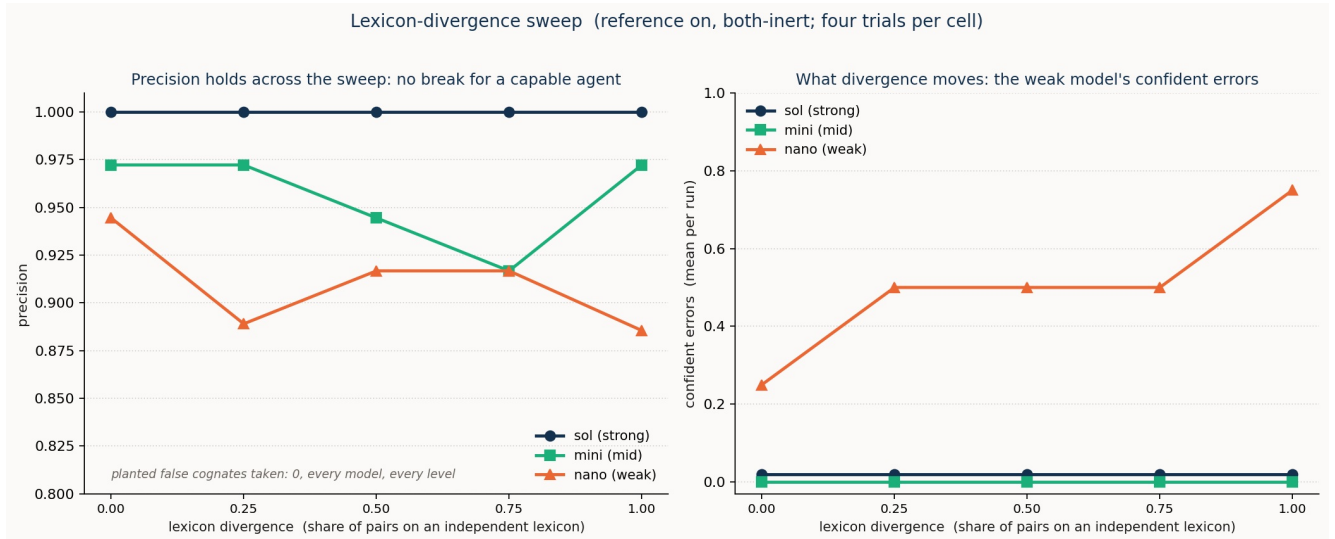
Figure 7. Left: precision across the divergence axis, per model. The strong agent is flat at 1.00, and no model takes a planted cross-lexicon false cognate at any level, so the guard itself never fails; the mid and weak agents vary in a narrow high band, spurious over-proposal rather than trap-taking. Right: the one quantity divergence moves is the weak model's confident-error count, which roughly triples across the sweep, while the stronger two stay at zero. Reference on, both-inert, four trials per cell.
