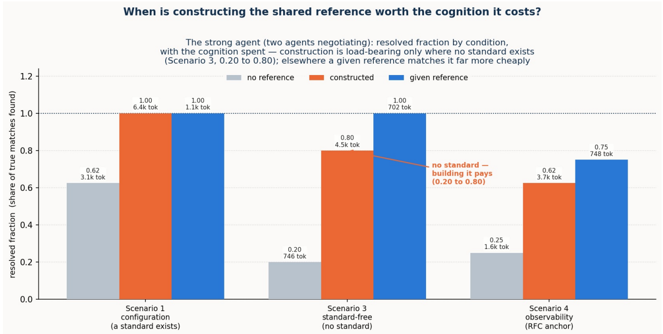
Figure 15 (when constructing a reference is worth it). The bars give the strong agent's resolved fraction under three reference conditions — no shared reference (grey), one the agents construct themselves (orange), and a given, already-published reference (blue) — across the schema scenarios, with the reasoning each condition spent noted on each bar. In scenario 3, where no standard exists, constructing the reference lifts the two agents from 0.20 to 0.80 (0.90 with a decisive experiment on the candidates) and is the realistic path; in scenarios 1 and 4 a given reference reaches the same close for a fraction of the cognition, so constructing one is redundant. Construction is capability-gated: a weak agent pays far more to build a worse reference, as the six-model ladder's non-convergence at the weak end shows.
