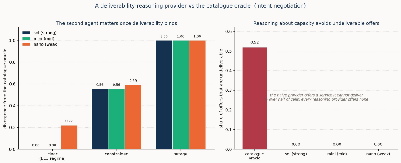
Figure 5.3. Left: the reasoning provider's divergence from the catalogue oracle by scenario, per model — near zero while paths are clear (the $5.1 fixed-catalogue regime) and rising as paths saturate and the provider must counter-propose or decline. Right: the catalogue oracle offers an undeliverable service in 0.52 of cells; every reasoning provider, across the ladder, offers none.
