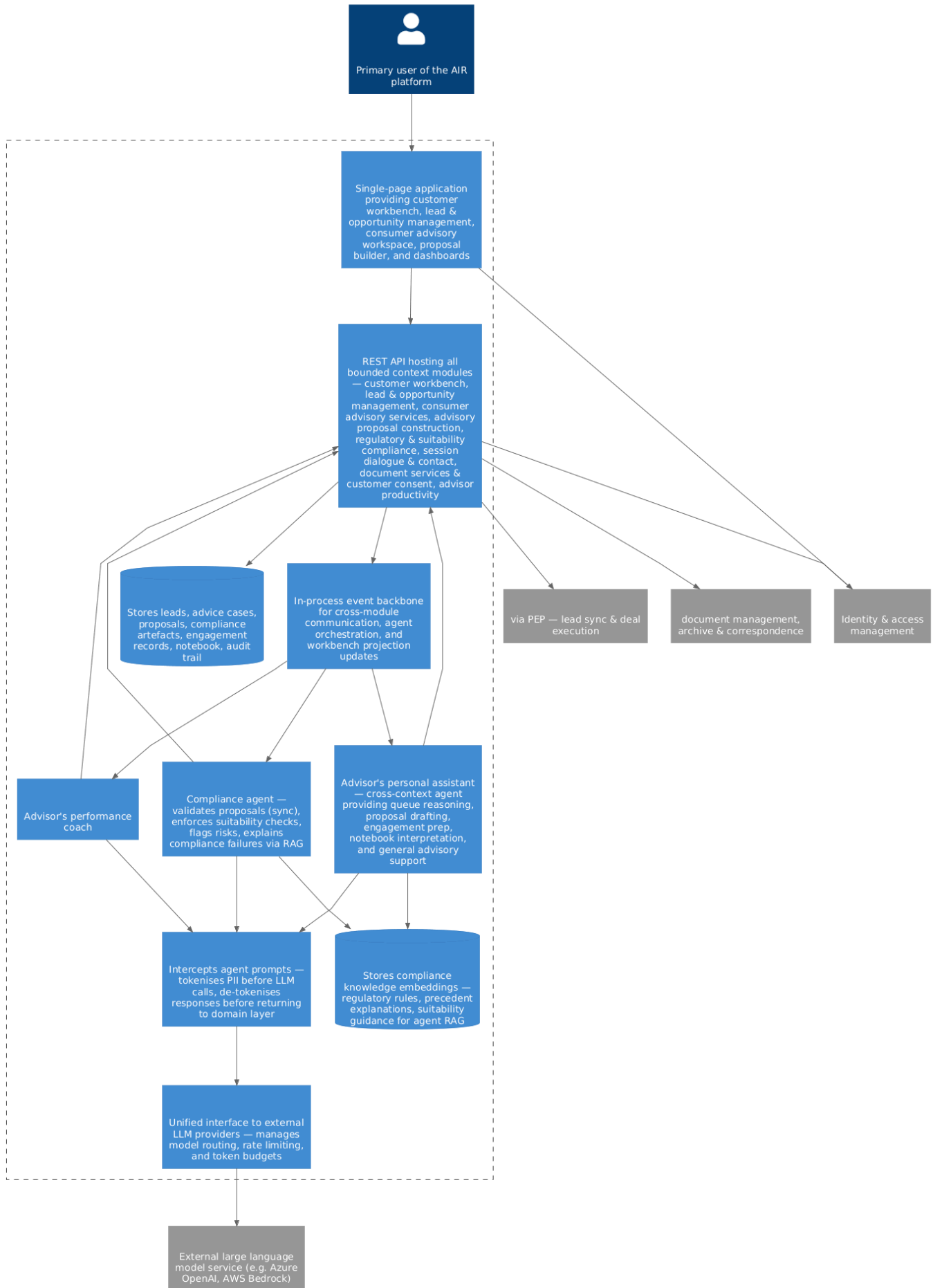
AIR Container Diagram
