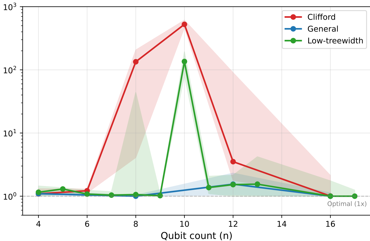
Overhead vs. fastest backend
