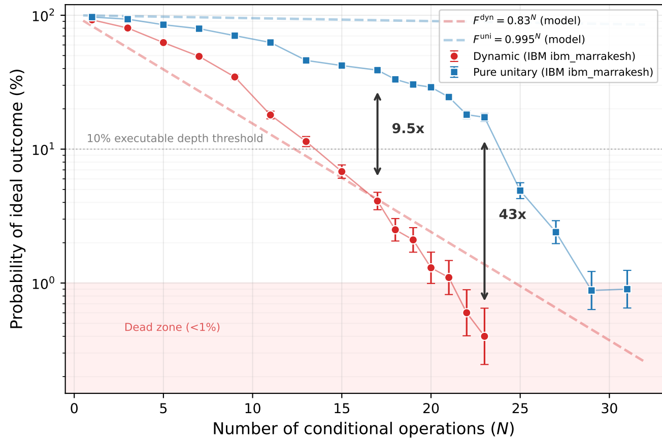
Experimental comparison: dynamic vs pure unitary circuits
