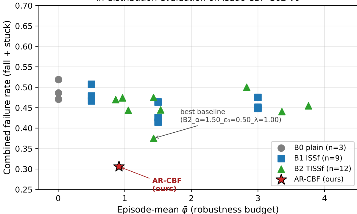
In-distribution evaluation on Isaac-CBF-Go2-v0
