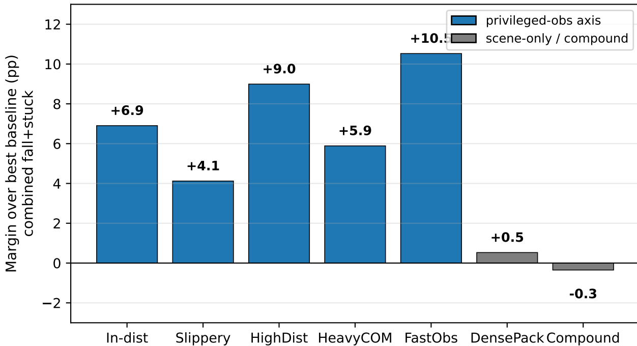
AR-CBF margin vs best hand-tuned baseline, per evaluation axis
