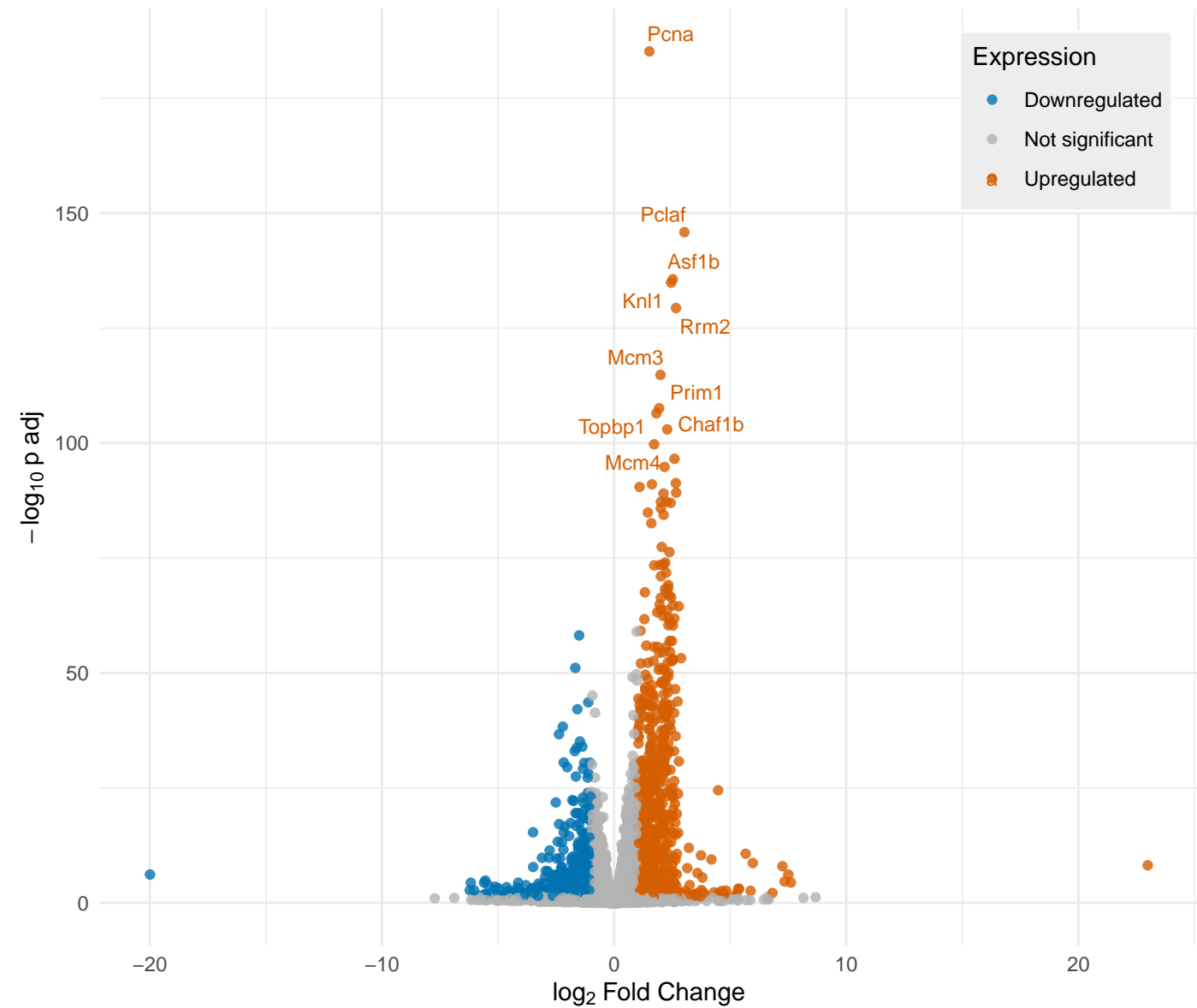
Differential Gene Expression: 24h Post-Reperfusion vs Control
