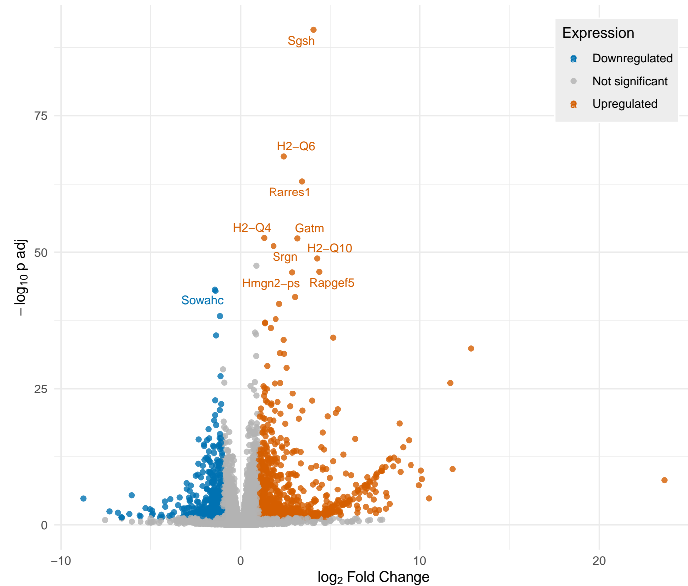
Differential Gene Expression: 2h Post-Reperfusion vs Control
