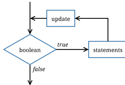
Figure 6.2: Flow of execution for a for loop.
