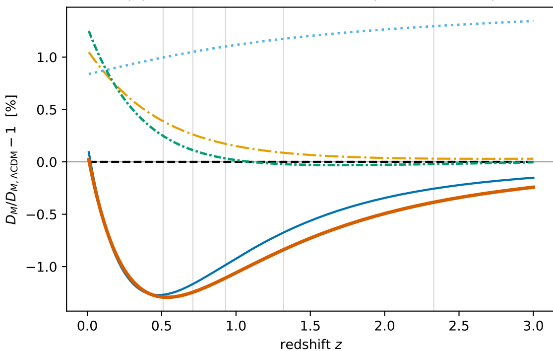
(3) Distance residual vs \Lambda CDM (DESI z shaded)
