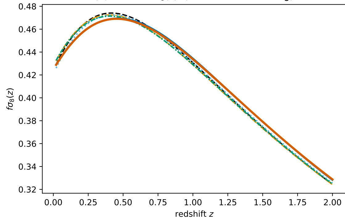
(4) Growth f\sigma_8(z) (GR, no DE clustering)
