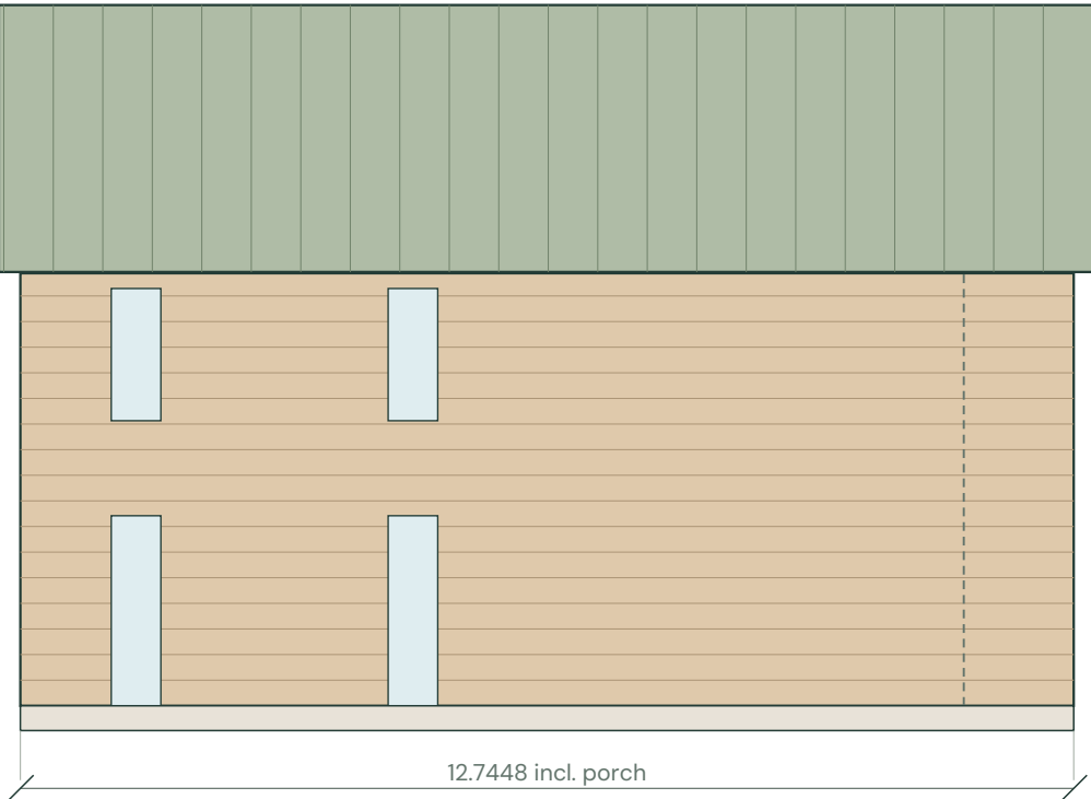
LEFT ELEVATION
