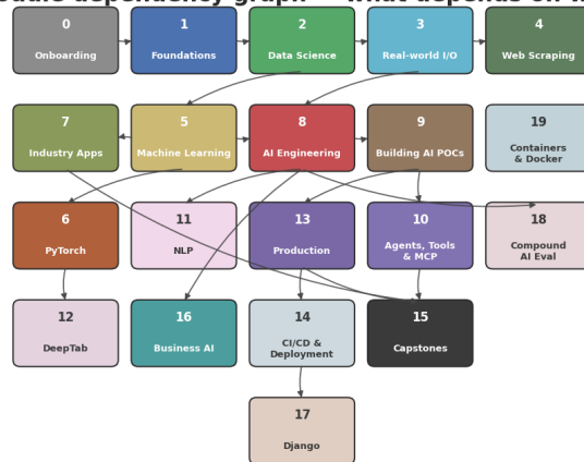
Module dependency graph — what depends on what
