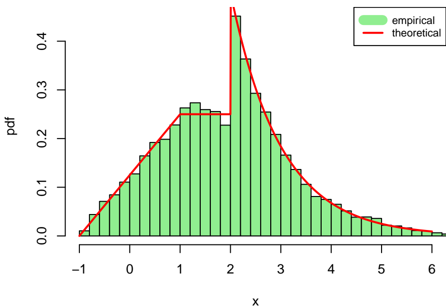
task3: rejection sampling (naive)
