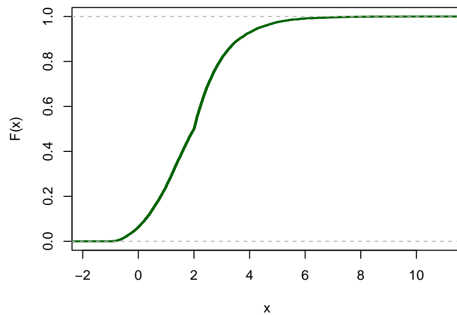
task3: cdf (naive)
