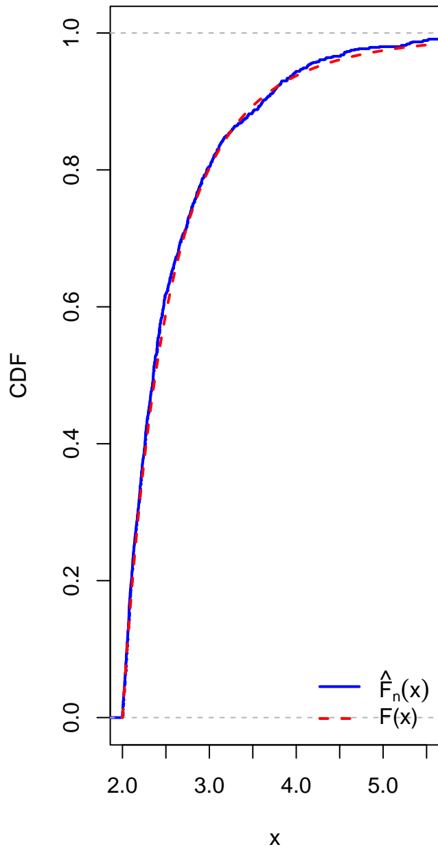
ECDF \hat{F}_n vs TCDF F(x)
