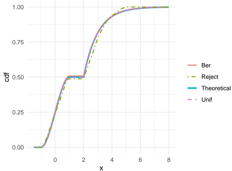
3 – CDF (Theoretical vs Ber/Unif/Reject)
