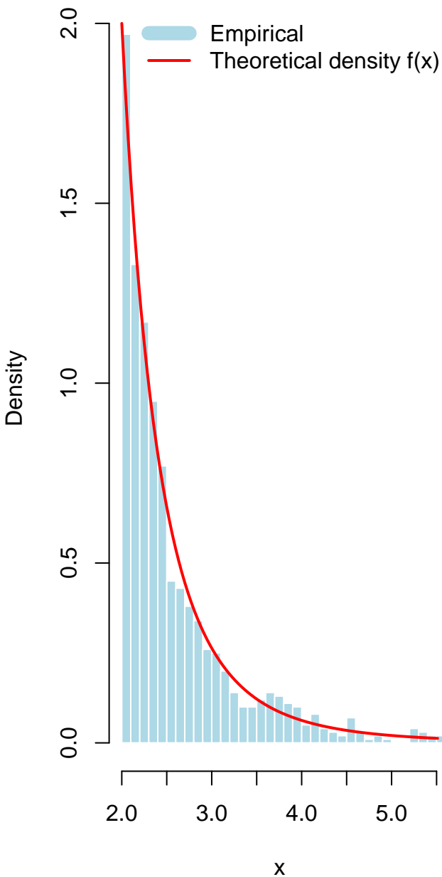
Histogram & f(x)
