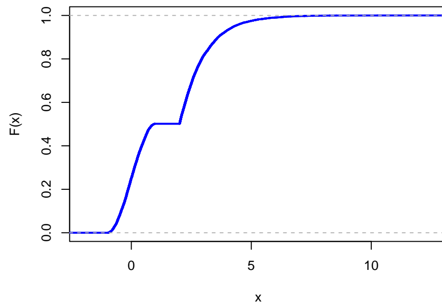
task2: cdf (naive)
