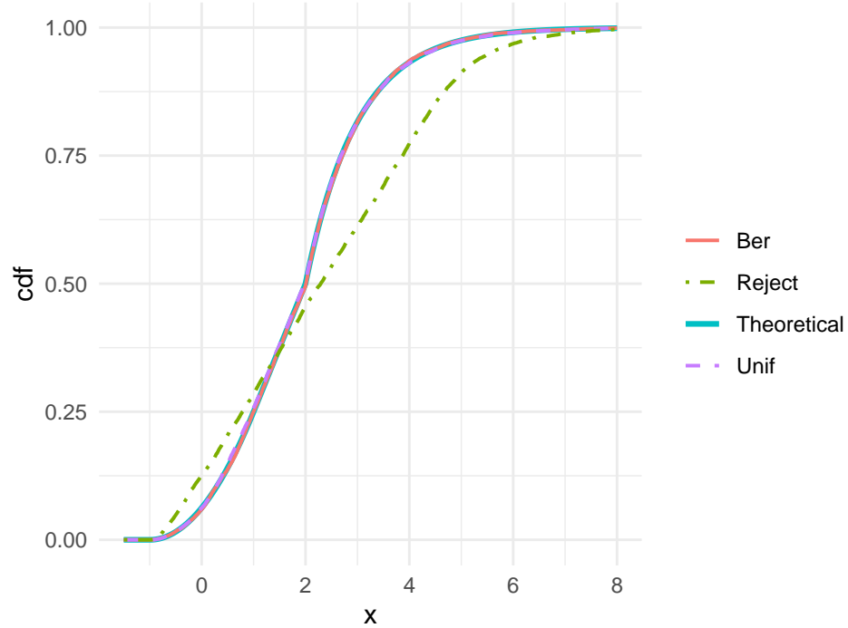
3 – CDF (Theoretical vs Ber/Unif/Reject)
