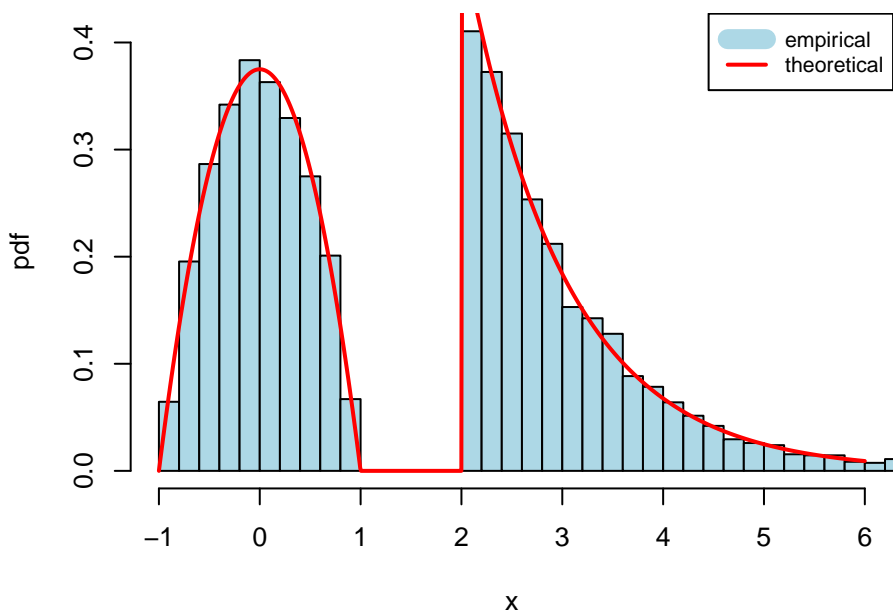
task2: rejection sampling (naive)
